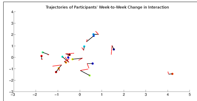
Figure 1: Visualization of change in interaction between weeks one and two (black) and weeks two and three (red).
