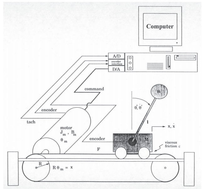
Figure 8: Schematic of classic inverted pendulum (Stimac 1999).
