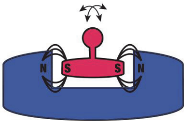
Figure 6: Electromagnetic pairs line the concentric walls of the EPS system. A pair consists of one electromagnet on the outer wall, and one ferromagnetic metal part on the inner wall.
