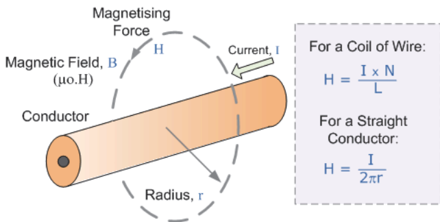
Figure 10: Generalized model of an electromagnet, like that proposed for EPS.
