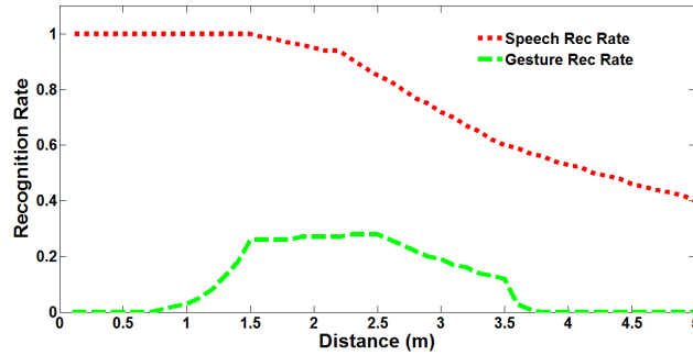
Fig. 6. Speech and gesture recognition rates as a function of distance.
