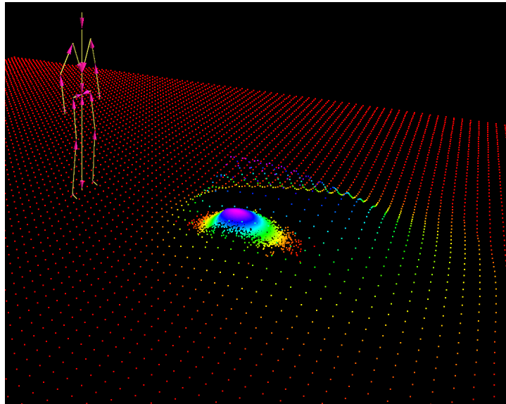
Fig. 10. Our autonomous sociable robot controller uses a sampling-based approach to estimate how the human produces social signals, and how the robot perceives them using models in our proxemic framework; a particle filter (with resampling) uses these estimates to maximize the expected performance of the robot during the interaction.
