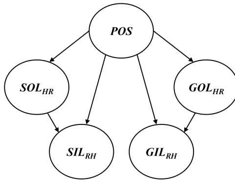
Fig. 2. A Bayesian network modeling relationships between pose, speech, and gesture.
