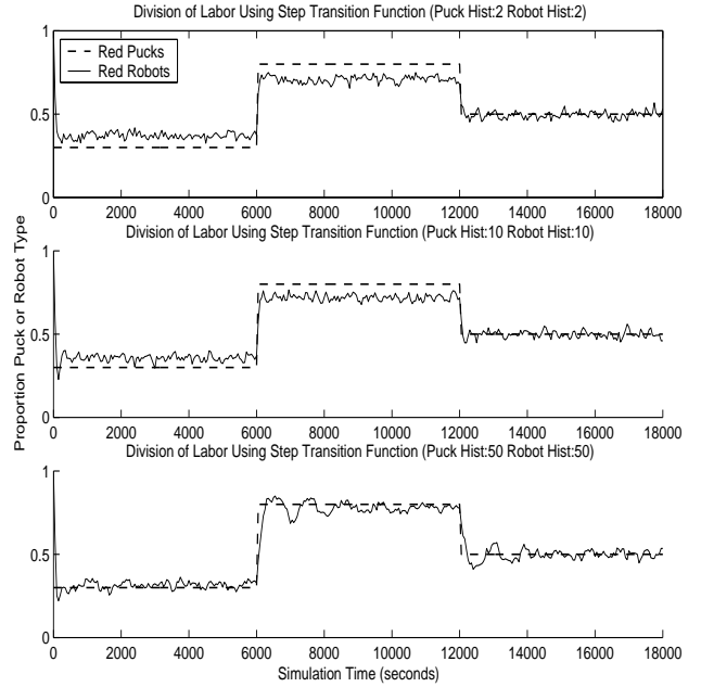
Fig. 2. The proportion of Puck Red pucks and robots foraging for Puck Red pucks over time when using the step transition function with different puck and robot history lengths.
