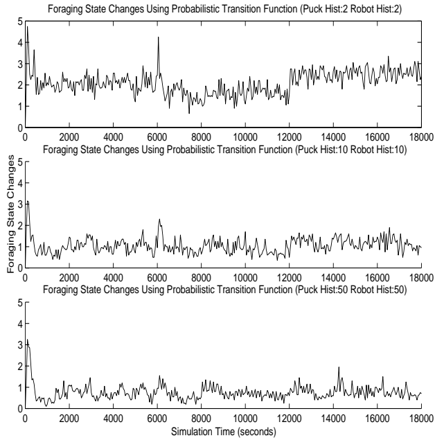
Fig. 5. The number of foraging state changes when using the probabilistic transition function with different puck and robot history lengths.
