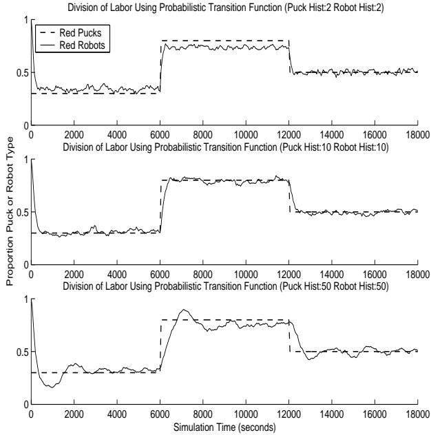
Fig. 3. The proportion of \text{Puck}_{Red} pucks and robots foraging for \text{Puck}_{Red} pucks over time when using the probabilistic transition function with different puck and robot history lengths.
