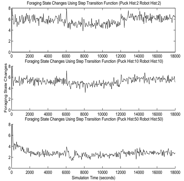
Fig. 4. The number of foraging state changes when using the step transition function with different puck and robot history lengths.
