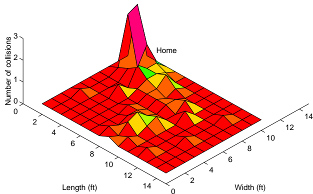
Fig. 6. This plot shows the characteristic interference pattern for the homogeneous implementation of the collection task on the four physical robots. The shading corresponds to the height of the peaks, best seen in color.
