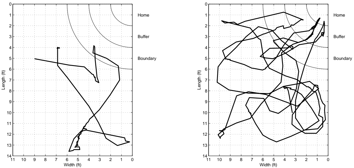
Fig. 17. (Left) A typical path of the least dominant robot of the pack controller; (Right) a typical path of the most dominant robot.
