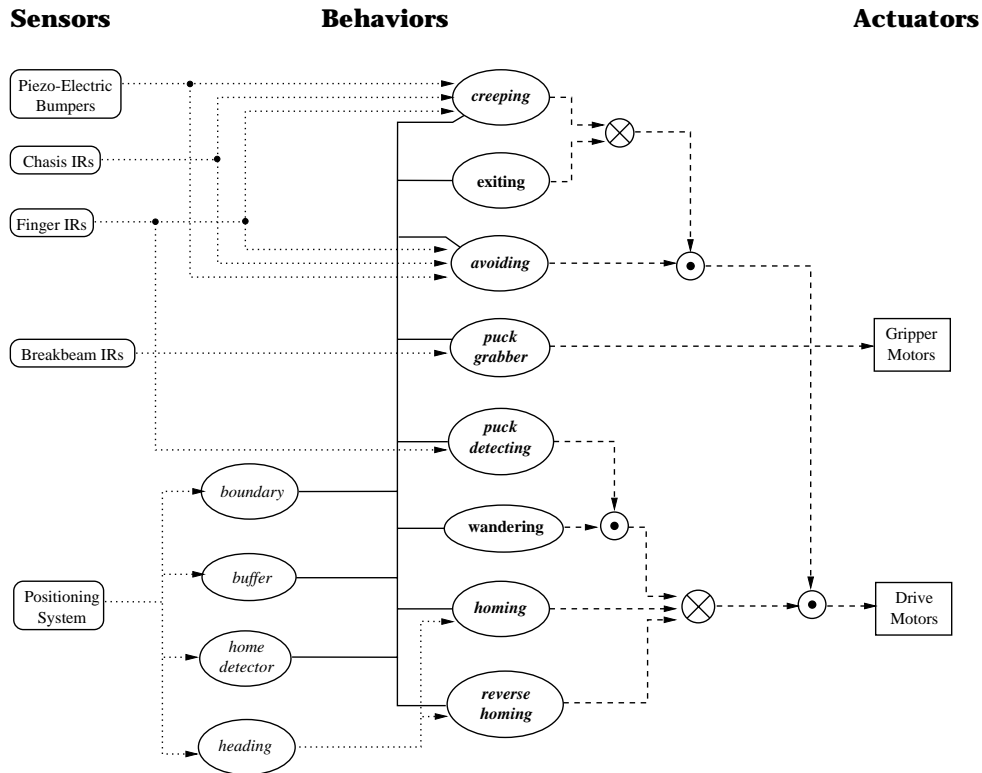
Fig. 5. The homogeneous controller for the collection task. Rounded rectangles represent the robot’s sensors, ellipses represent behaviors, and rectangles represent actuators. Sensor values are transmitted along dotted lines, actuator commands along dashed lines, and inter-behavior control signals along solid lines. The \otimes represents behavior selection and the \odot represents Subsumption-style precedence.
