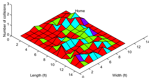
Fig. 14. This plot shows the characteristic interference pattern for the caste implementation of the collection task on the four physical robots. The shading corresponds to the height of the peaks.
