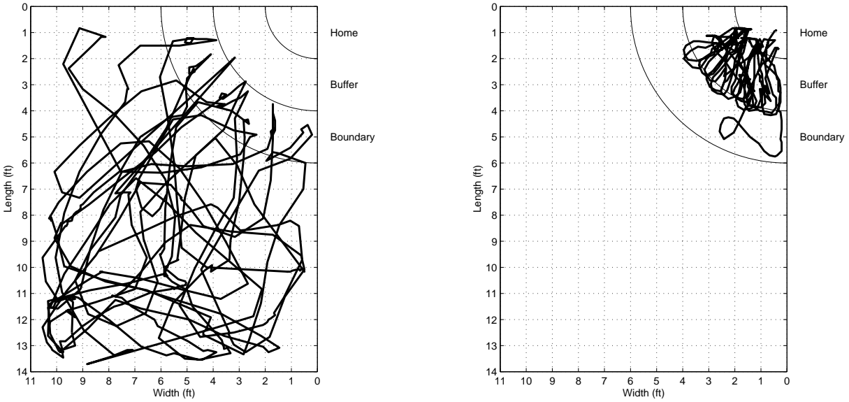
Fig. 16. (Left) A typical path of a physical robot in the Search Caste of the caste controller; (Right) a typical path of the robot in the Goal Caste.
