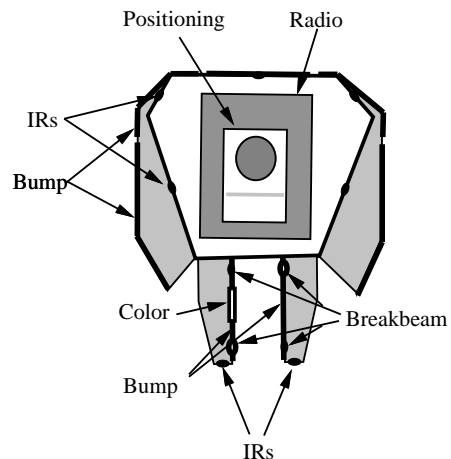
Fig. 4. The sensor configuration of an R2e robot.
