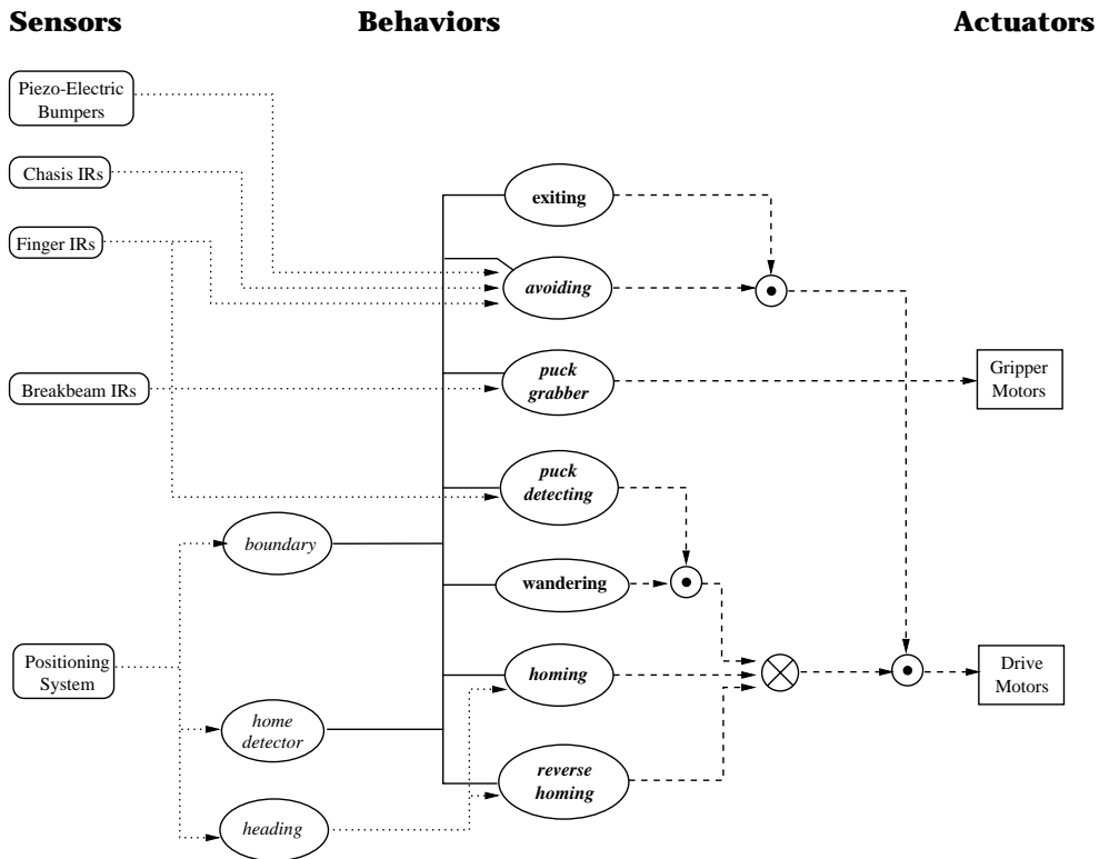
Fig. 11. The controller for the Search Caste, the three robot subgroup that searches for pucks.
