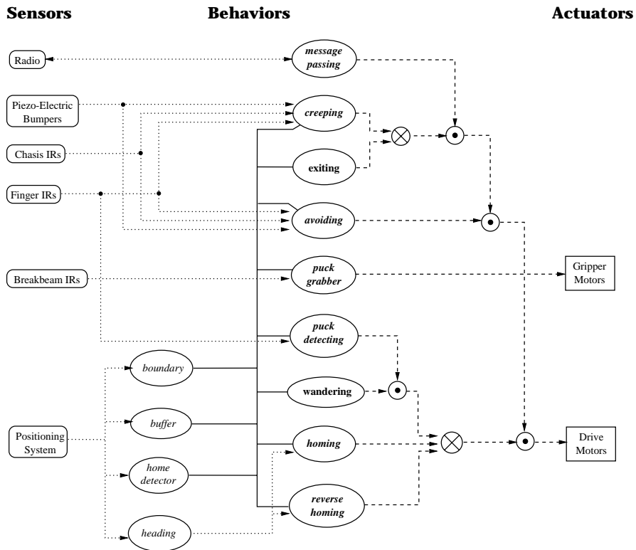
Fig. 8. The pack version of the controller for the collection task.
