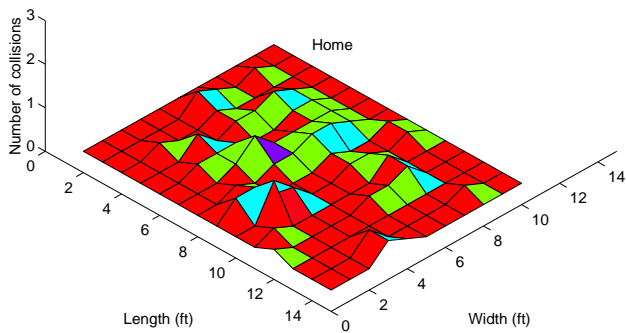
Fig. 9. This plot shows the characteristic interference pattern for the pack implementation of the collection task on the four physical robots. The shading corresponds to the height of the peaks.
