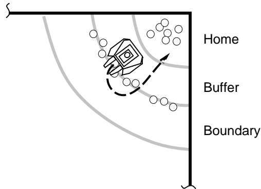
Fig. 12. The sweeping behavior of the controller for the Goal Caste.
