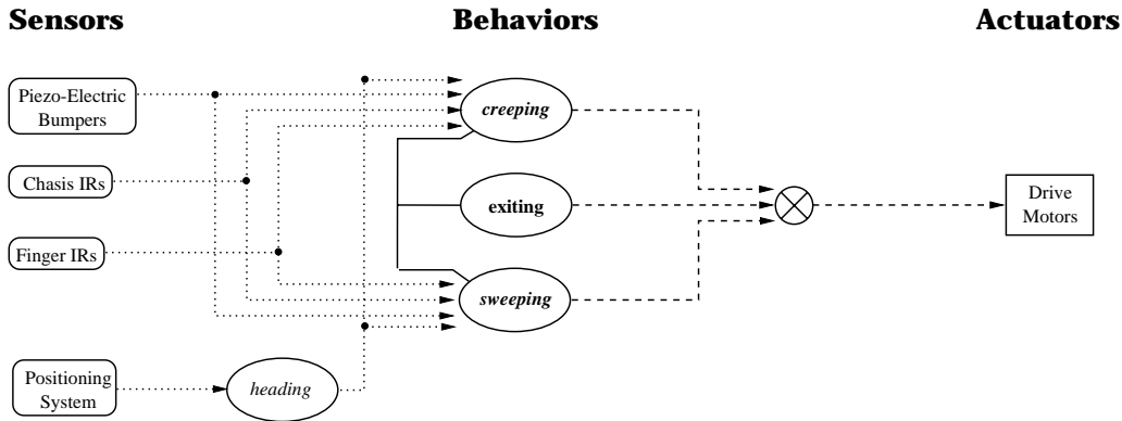
Fig. 13. The controller for the Goal Caste, the one robot subgroup that brings pucks from the Boundary/Buffer line to Home.
