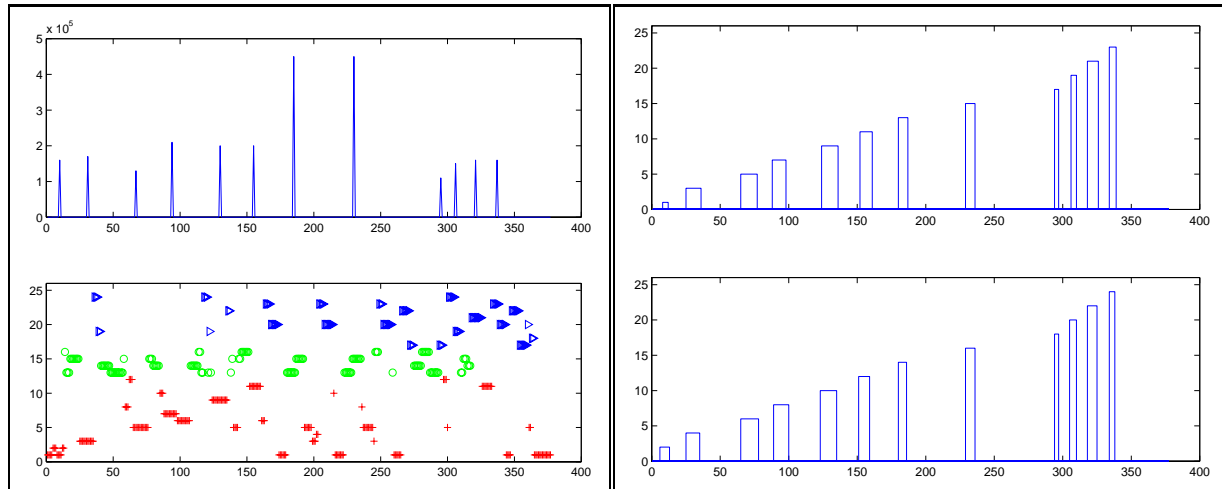
Fig. 7. The results from classification of the training motion for the right and left arms. Left: plots of L(t) (above) and Q(t) (below) corresponding to the maximum valued response and active perceptual description for the left end-point with respect to time. In the plot of Q(t) , Q(t) identifies the index of the active description, these indices are separated into crosses for lines, circles for circles, and triangles for arcs. Right: plot of Q(t) for the left and right arms after thresholding for valid segments.
