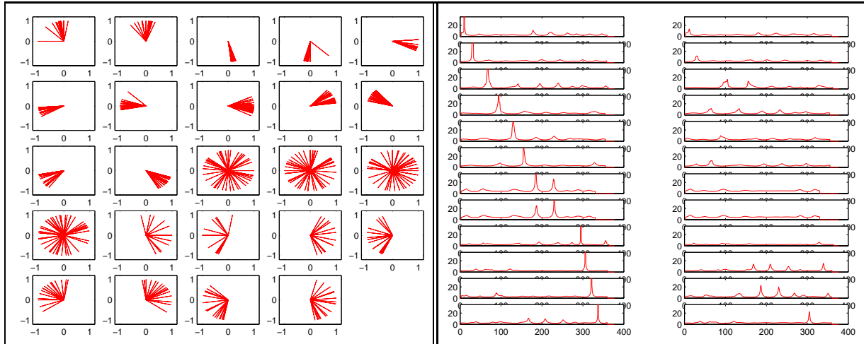
Fig. 6. Left: The set of normalized gradients in (x,y) space for each of the primitive instances, consisting of 12 line, 4 circle, and 8 arc instances in left to right order. Right: The response R(t) over time for the movement of the left end-point against the manually determined primitive set. The left and right columns present the response to the left and right arm perceptual descriptions, respectively. The first six rows represent line primitive instances, the next two rows are circle instances, and the last four rows are arc instances.
