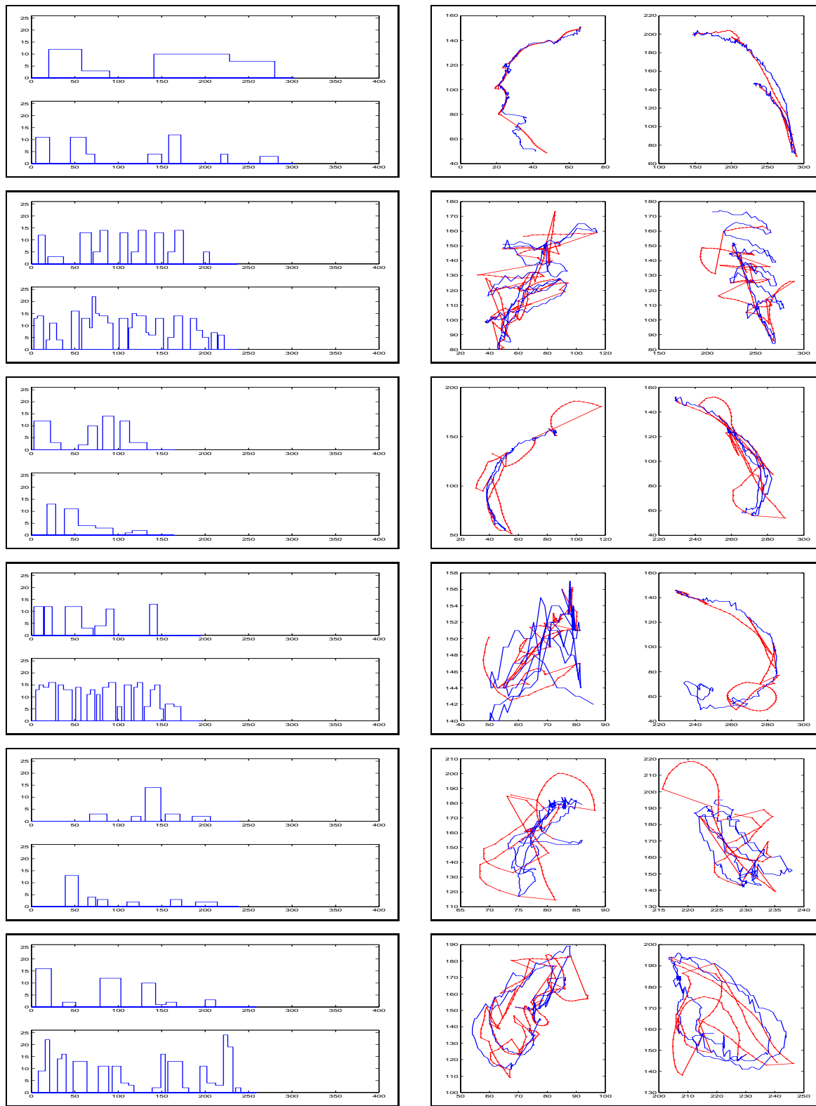
Fig. 12. The rows of this figure provide the segments that result from classification and the reconstructed end-point trajectories for our set of test motion. The y-axis of the segmentation plots are the indices of the perceptual descriptions. The rows show the results for throwing, aerobic arm thrusts, alternating waves, "egyptian", and two versions of "raising the roof".
