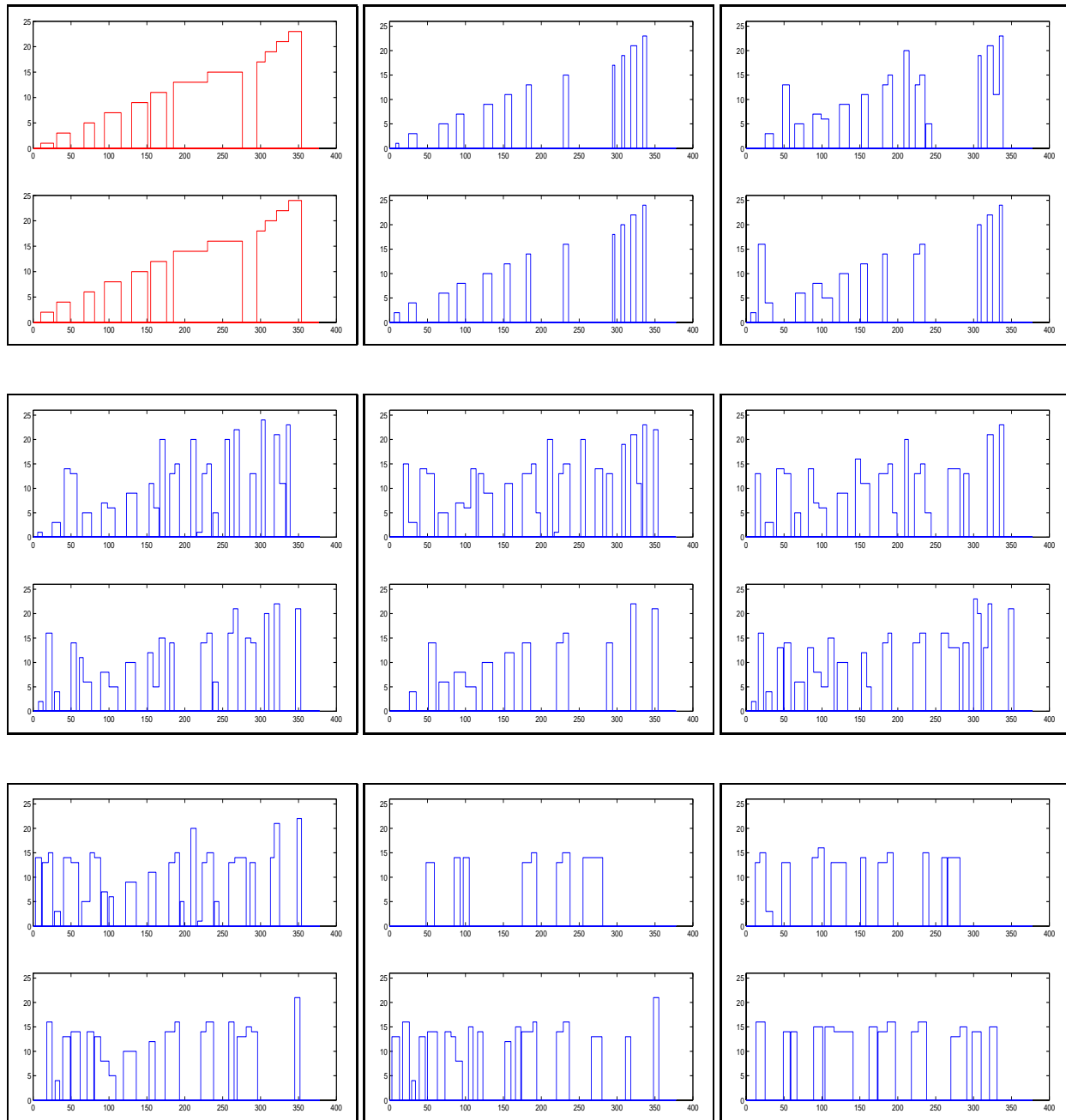
Fig. 11. The upper left plot shows the manual segmentation of the training motion into the primitive descriptions for the left and right end-points. The succession of plots from left to right and top to bottom show the result after segment validation for distortions of increasing noise level corresponding to 0, 1, 3, 5, 7, 9, 15, and 25.
