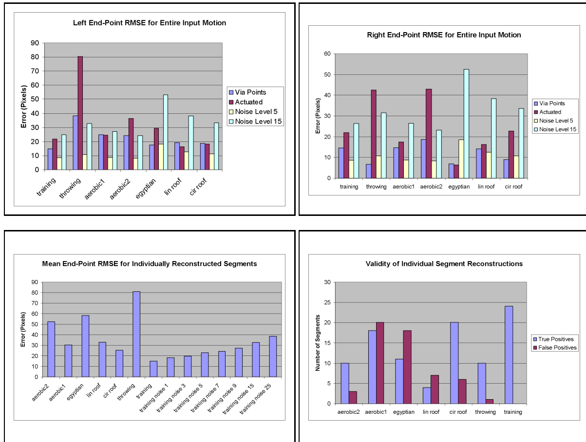
Fig. 9. Plots of evaluations for entire motion RMS error, mean individual RMS error, and individual segment validity.
