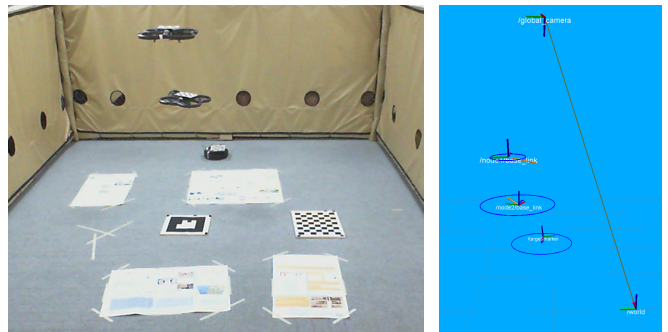
Fig. 2. Two AR.Drones tracking the target – currently in a string topology. The state estimates are shown as blue arrows, the corresponding covariances are represented by blue ellipses. The commanded velocities are shown as orange arrows.
