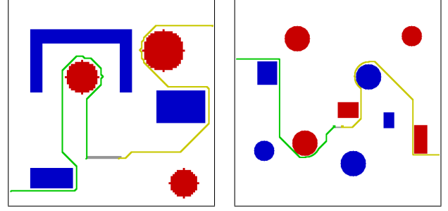
(a) The planned trajectories in a 100 \times 100 discretized environment. (b) The planned trajectories in a 400 \times 400 discretized environment. Fig. 7. Decoupled, distributed plans. Initial cable is shown in gray/black. Trajectories are in green and yellow.
