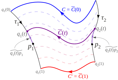
Fig. 3. Illustration for Proof of Prop. 2.
