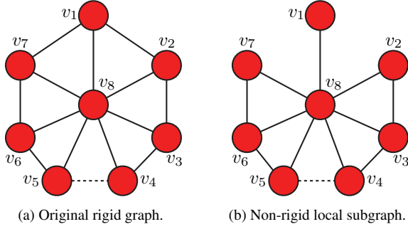
Fig. 4. An illustration of conservatism in the local redundancy rule. The edge (v_4, v_5) is redundant with respect to graph (a). However, applying the local redundancy check over subgraph (b) suggests (v_4, v_5) is independent (due to non-rigidity), denying link deletion.
