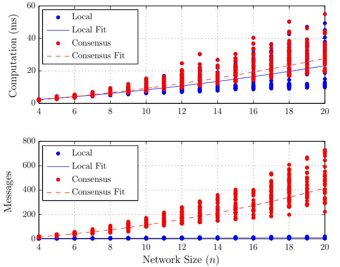
Fig. 5. Monte Carlo simulations comparing computation and communication complexity versus network size ( n ) for our proposed local rule and the consensus-based extension.
