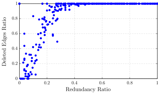
Fig. 6. Monte Carlo simulations demonstrating conservative behavior of the local rigidity rule for link deletions, measuring redundancy versus deleted edges.
