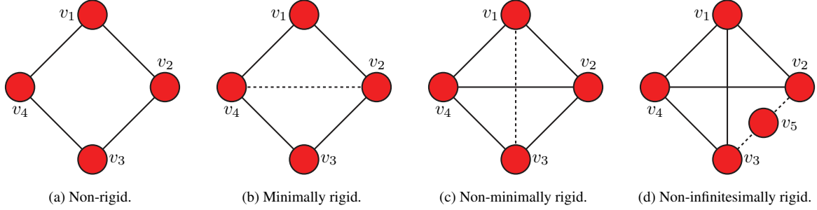
Fig. 1. Example graphs demonstrating several embodiments of rigidity, where dashed links indicate edges that have been added to form new networks. Notice that all links in graphs (a), (b), and (d) are independent, while edge (v_1, v_3) in (c) is redundant.
