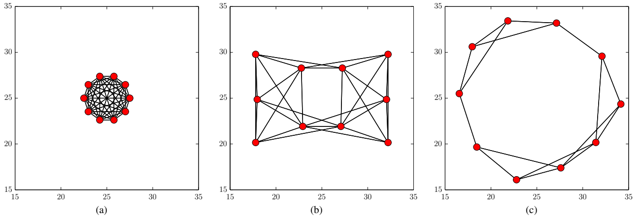
Fig. 6. Dispersion simulations of an n = 10 agent system with interaction model \rho_2 = 10 , \rho_1 = 7 , and \rho_0 = 2 , under minimum degree constraints |\mathcal{N}_i| \geq 5 [(b)] and |\mathcal{N}_i| \geq 3 [(c)]: (a) initial fully connected ring network configuration; (b) final converged configuration |\mathcal{N}_i| \geq 5 ; and (c) final converged configuration |\mathcal{N}_i| \geq 3 .
