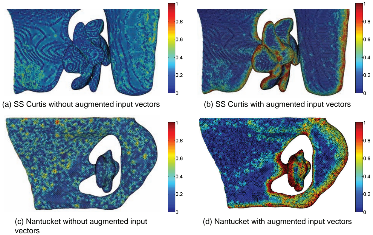
Fig. 4. Comparison of normalized uncertainty on the surface of the SS Curtiss (top) and Nantucket Lightship (bottom) meshes using a squared exponential kernel without augmented input vectors (left) and with augmented input vectors (right). Red areas are high uncertainty, and blue areas are low uncertainty. The areas of high variability have higher uncertainty when the augmented input vector is used. This figure is best viewed in color.
