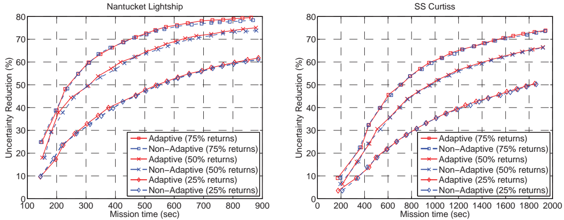
Fig. 8. Mission time versus expected uncertainty reduction for inspection simulations with different levels of stochasticity in the sensor model. The non-adaptive strategy provides competitive performance with the adaptive strategy, as predicted by the small adaptivity gap.
