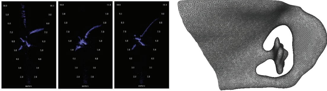
Fig. 3. An example of the raw data, and subsequent result, of the surface construction procedure. At left, three range scans featuring the hull, propeller, and rudder of the Nantucket Lightship, a historic ship 45 m in length. These scans were collected in sequence as the HAUV dove with the running gear in view. At right, a 3D triangle mesh model from the complete survey of the Nantucket Lightship.
