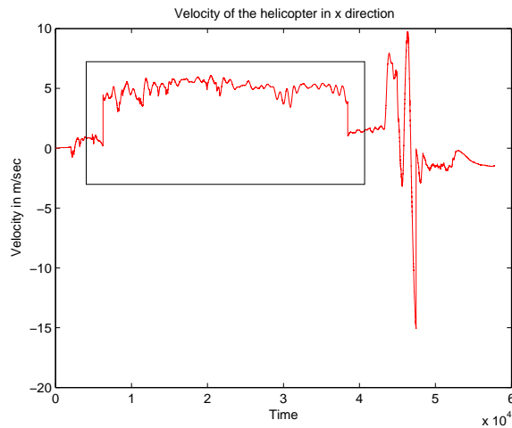
(a) Helicopter velocity in lateral direction. The box represents the region of interest. The velocity stays constant for the entire tracking period as predicted in section II
