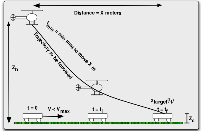
Fig. 4. Schematic for landing on a moving target
