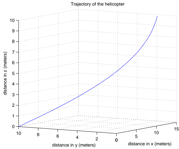
(a) Trajectory of the helicopter
