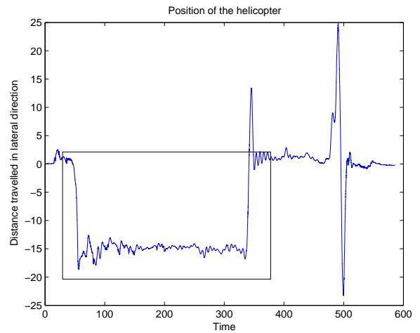
(b) Position of the helicopter in the lateral direction. The box shows the time during which the helicopter follows a straight line trajectory
