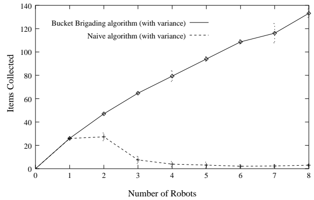
Figure 8: Experiment 1a (2a), Narrow corridors
