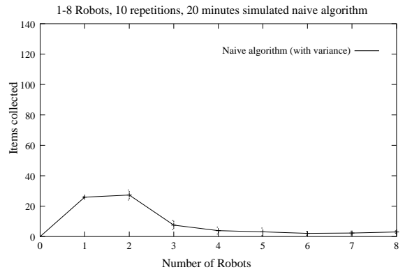
Figure 6: The performance of the naive algorithm, 1-8 robots, 10 repetitions of 20 minute runs, in the maze like environment.
