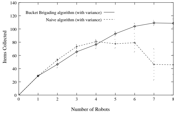
Figure 9: Experiment 1b, Less narrow corridors
