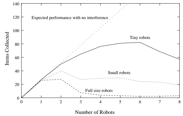
Figure 13: Naive algorithm performance, 2a-2c
