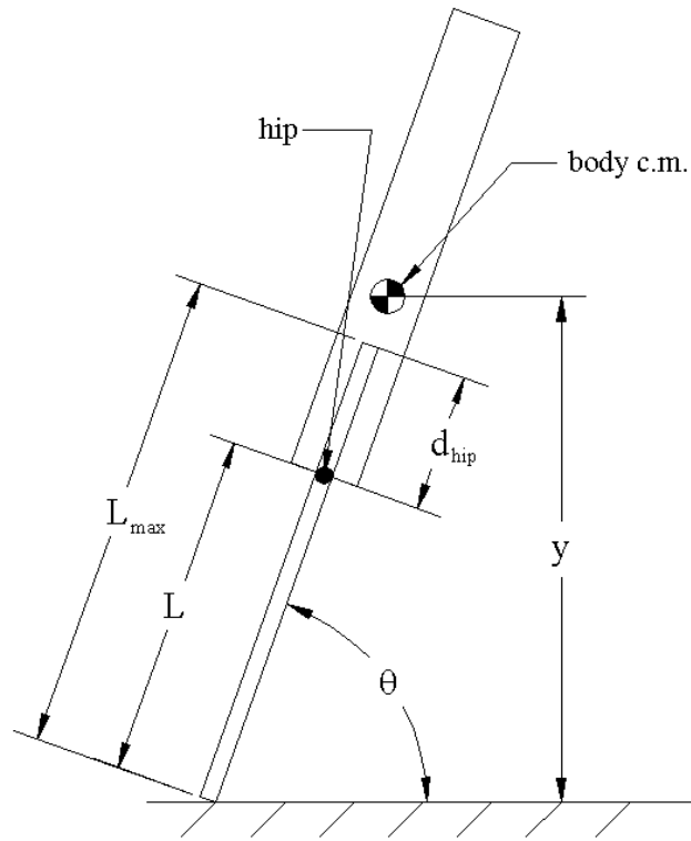
Fig. 2. 2d hopping machine in stance. The body is not shown.
