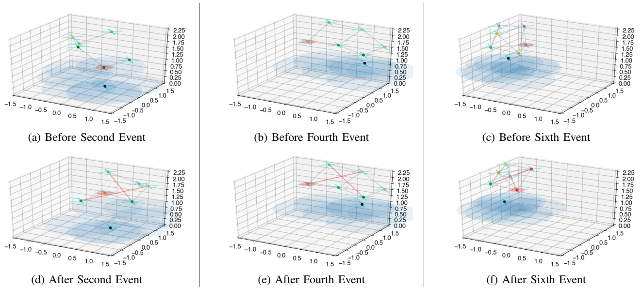
Fig. 4: Screenshots of a simulation in which a six quadrotor team tracks another quadrotor flying below them. The tracking team’s sensing area is colored in light blue. The figures in the top row depict the formation of the quadrotors before the occurrence of a sensor deterioration event. The corresponding figures on the bottom portray the formation after 1) sensor deterioration is detected, 2) a new communication edge is chosen, and 3) the robots move to their new locations. The quadrotor which experienced sensor deterioration is enveloped using a filled red circle. The quadrotor colors vary from green to red indicating good to poor sensor quality. For visualization purposes, we set n_e = 2 for this simulation to illustrate multiple edges added for deterioration events. We also set d_s = 0.5 , d_{mc} = 1.0 , and d_{sen}^i = 1.0 \forall i \in [n] , with a bounding box of x \in [-1.5, 1.5] , y \in [-1.5, 1.5] , and z \in [1.6, 2.25] .
