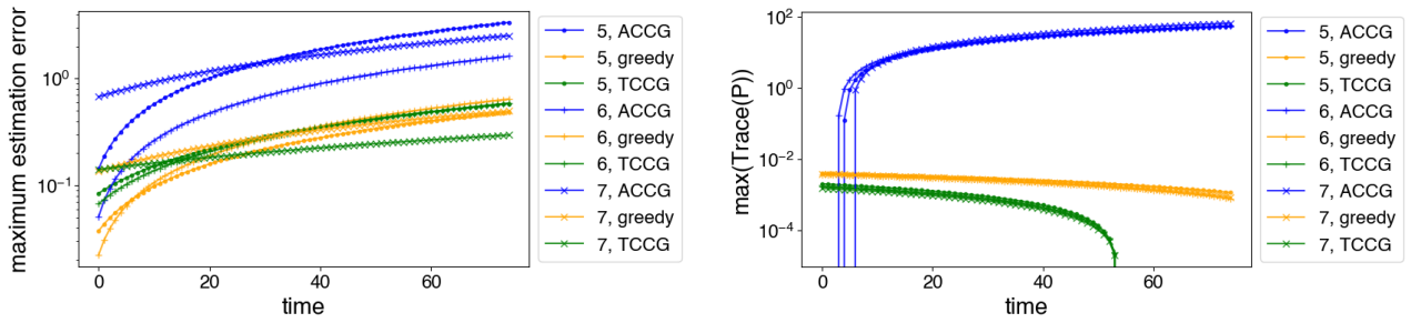
Fig. 5: The comparison (log scale) of maximum estimation error and maximum Tr(\mathbf{P}) for all simulations and all team sizes between ACCG (blue), TCCG (green), and the greedy approaches (orange). TCCG performs better over time in terms of estimation error for teams of n = 6 and n = 7 . TCCG also performs best in terms of the trace of the covariance matrix for all team sizes.
