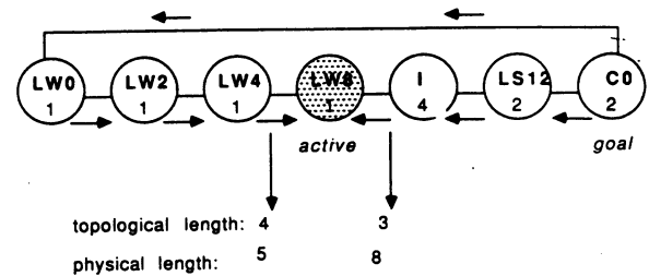
Fig. 12. The graph the robot constructed of the shown environment. Shaded nodes indicate the robot's current location and the goal, and the arrows indicate the direction of activation propagation. To test the robot's ability to use the correct measure of optimality, the corridor was chosen as the goal when the robot was located at LW8. The topologically shortest path involves going through a cluttered area with a long irregular boundary. Consequently, the robot consistently chose the topologically longer but physically shortest path around the room.
