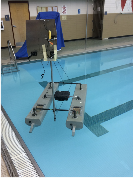
Figure 2: Image of the employed experimental setup for swimming pool testing. A stereo camera is maintained at a constant altitude above the water’s surface with a catamaran platform. Parallel laser beams are used to provide scale throughout the water column.
