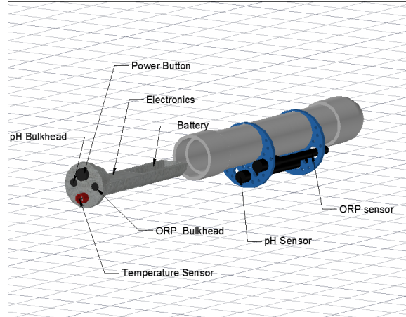
Fig. 9. The general layout of the inner cylinder is shown above.
