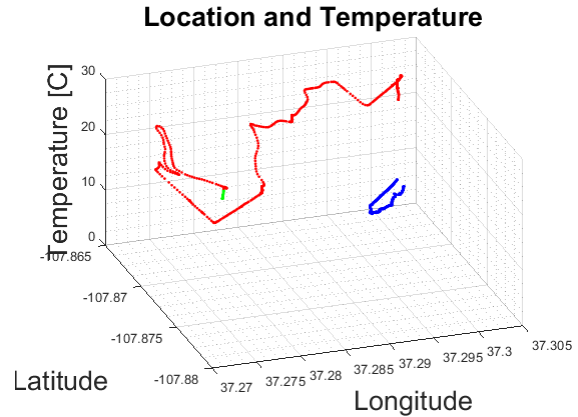
Fig. 15. Corresponding temperature versus GPS location for the testing on April 25, 2016 is shown.
