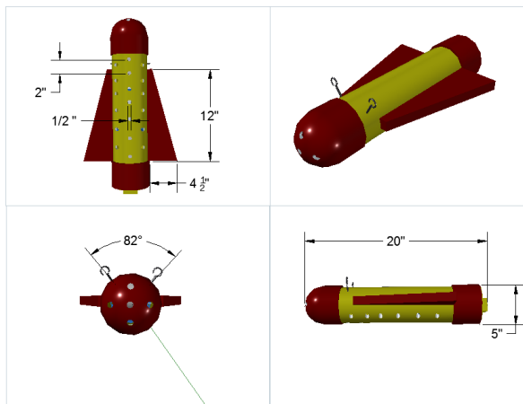
Fig. 8. A protective outer cylinder with holes was used to house the inner cylinder.
