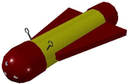
Fig. 2. CAD model of the fully-assembled, water sampling prototype.
