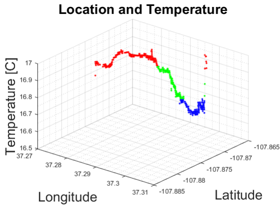
Fig. 17. Corresponding temperature versus GPS location on the Animas River on July 15, 2016 is shown.
