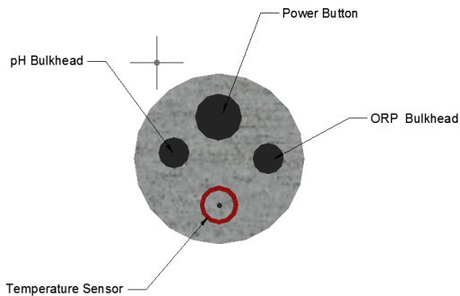
Fig. 11. Cap layout for the inner cylinder.
