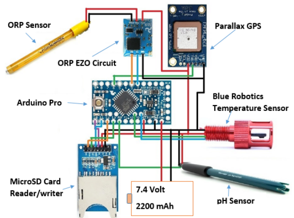
Fig. 12. The wiring diagram for the electronics that measure temperature, pH, GPS, ORP, and velocity is shown above.
