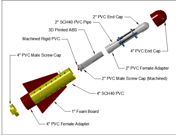
Fig. 10. A protective outer cylinder with holes was used to house the inner cylinder.
