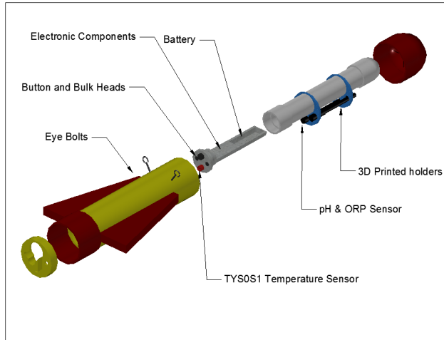
Fig. 7. Electric components were mounded on a 3D printed plastic platform that was placed inside an inner cylinder within an outer cylinder.
