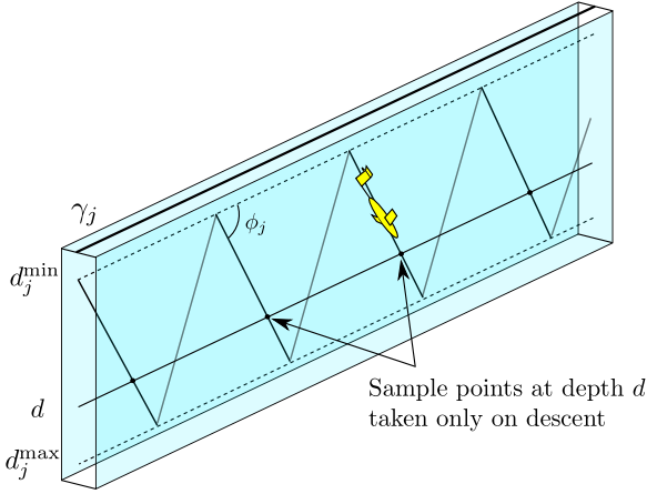
Fig. 5. The sawtooth pattern that the glider follows along each path segment \gamma_j is shown with its relevant parameters labeled. The sawtooth pitch \phi_j controls the sample density, which we define as the number of samples per distance at a fixed depth d .
