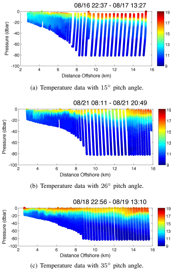
Fig. 6. Pressure vs. Distance from Shore plots of Temperature ( ^{\circ}\text{C} ) data collected along the same transect for 6(a) 15^{\circ} , 6(b) 26^{\circ} and 6(c) 35^{\circ} . Individual measurements are shown to emphasize the sampling resolution along each path. Start and end times for the transect are shown above each respective figure, with the year assumed to be 2010.
