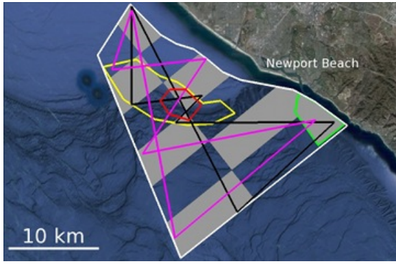
Fig. 4. This figure presents an enlarged view of Figure 3 with the glider paths overlaid. The path produced by the ZZTOPP Algorithm is given by the black line, while the magenta line represents the reference path that was hand-delineated by an oceanographer to survey the same region with the same constraints. The mission domain Q is delineated by the white polygon. Regions Q_1 , Q_2 and Q_3 are the high interest regions, and are delineated by the red, green and yellow polygons, respectively. The grey shaded polygons denote the checkerboard regions.
