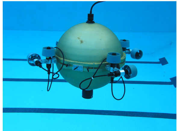
Figure 1. ODIN operating in the pool.
