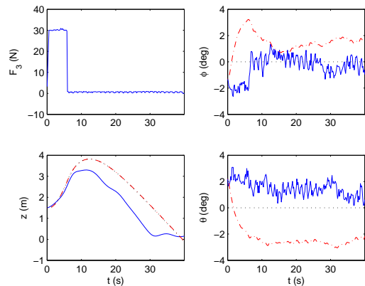
Figure 2. Pure Heave Motion of 2.3m.
