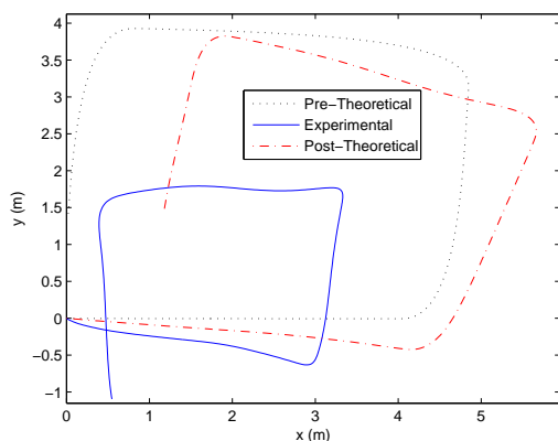
Figure 4. Ad Hoc Rectangle Trajectories.
