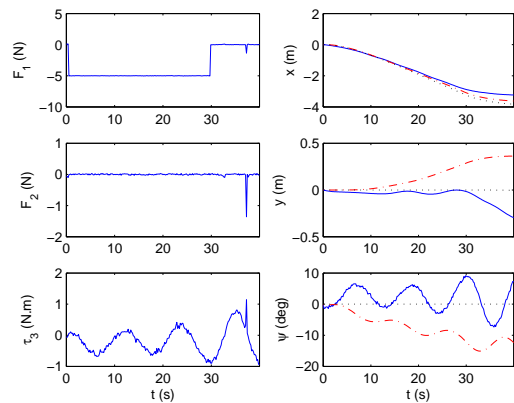
Figure 3. Pure Surge Motion.
