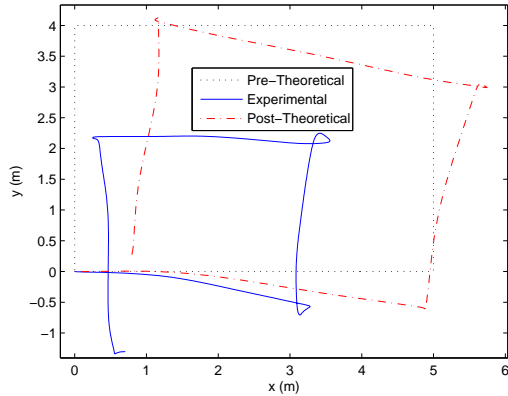
Figure 5. Calculated Rectangular Trajectories.
