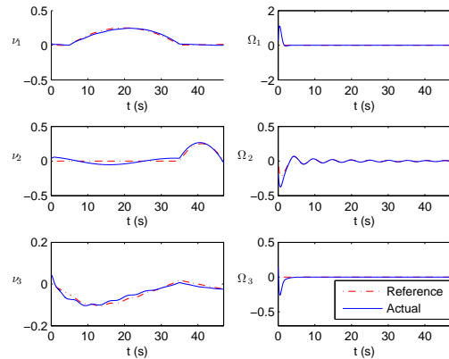
Figure 8. Comparison of the Reference and Actual Velocities of the AUV (Mission 2)
