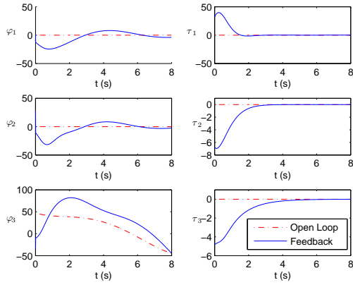
Figure 4. Comparison of the Control Effort in Feedback scheme as compared to the Open-Loop scheme (Mission 1)
