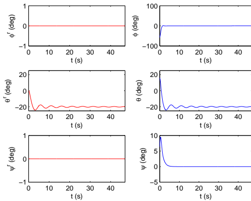
Figure 7. Comparison of the Reference (\cdot)^r and Actual Euler Angles of the AUV, (Mission 2)
