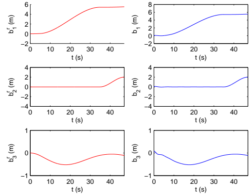
Figure 6. Comparison of the Reference( b_j^r ) and Actual( b_j ) Position of the AUV, (Mission 2)
