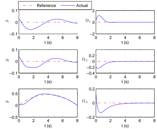
Figure 3. Comparison of the Reference and Actual Velocities of the AUV (Mission 1)
