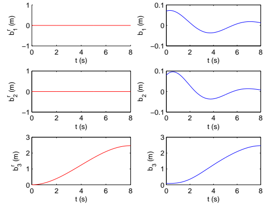
Figure 2. Comparison of the Reference( b'_j ) and Actual( b_j ) Position of the AUV (Mission 1)
