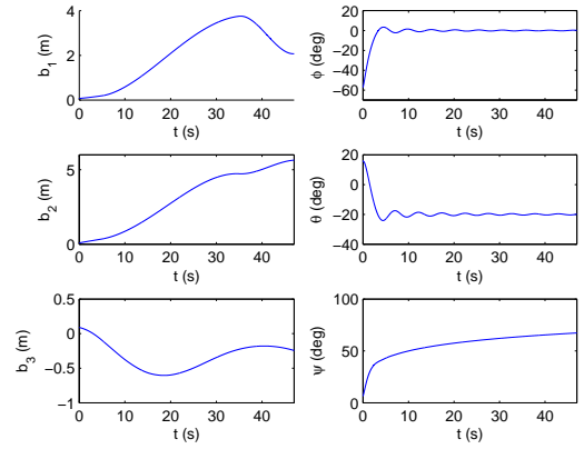
Figure 5. Position and orientation using open-loop control with initial disturbances (Mission 2)
