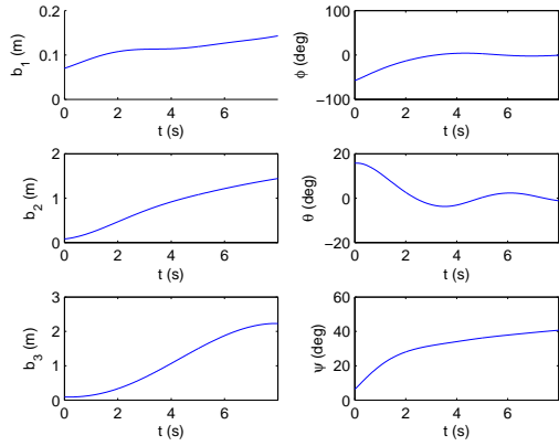
Figure 1. Positions and orientations using open-loop control with initial disturbances (Mission 1)
