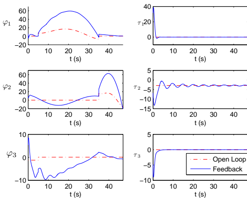
Figure 9. Comparison of the Control Effort in Feedback scheme as compared to the Open-Loop scheme (Mission 2)
