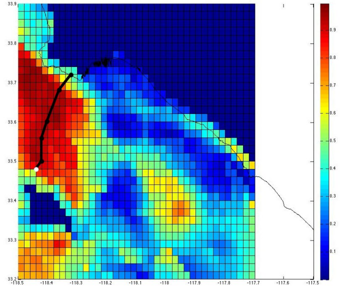
(a) Controllability map generated from ocean model predictions. Blue refers to areas of low controllability, and red are areas of high controllability.
