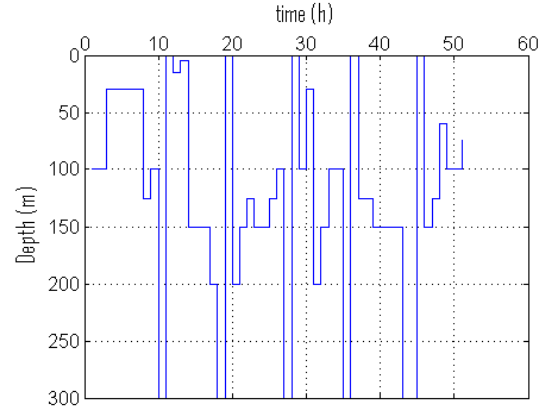
Fig. 4. A plot of the prescribed depth of the float versus time as computed by the RCFMPC.
