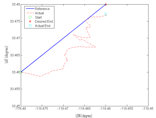
Fig. 5. The path followed by the profiling float (dashed red line) by executing the control presented in Fig. 4. The prescribed path is given by the solid blue line.
