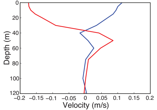
Fig. 2. An example vertical current profile prediction for a location off the coast of southern California, USA. This is a ROMS prediction of ocean depth versus current velocity for the zonal (blue) and meridional (red) components located at 33.5^\circ N, -118^\circ E.
