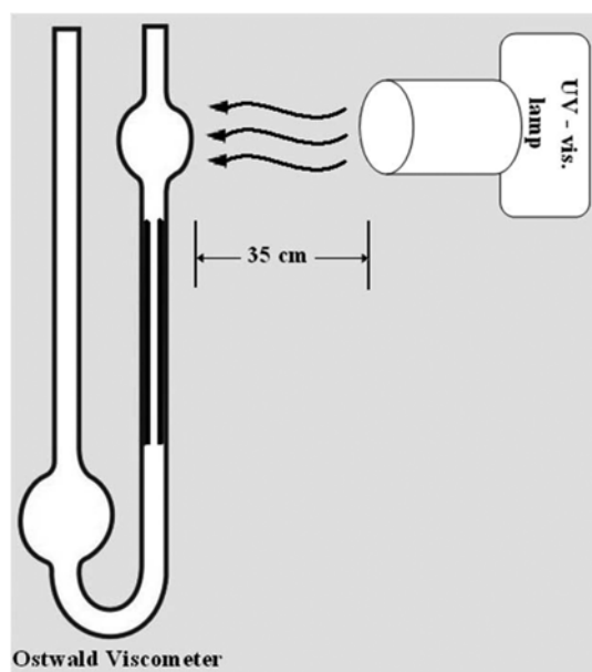
Fig. 1. Depiction of experimental setup used for determining photoinduced rheological effects on titania suspensions in conducting and insulating mediums.
