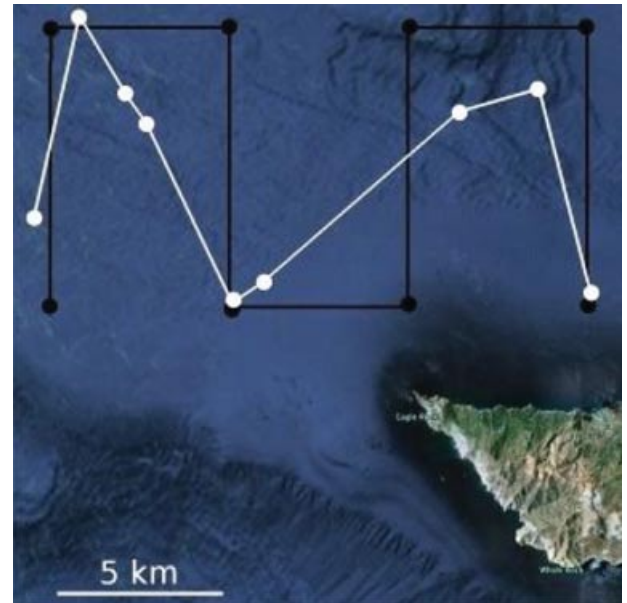
Figure 2. Planned lawn mower pattern (black waypoints and path) and the actual executed path (white surfacing locations and path) for a glider deployment off the northern tip of Santa Catalina Island, California.
