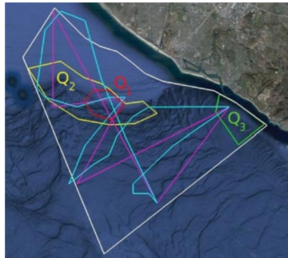
(b) Computed path for the second SCB deployment (magenta line) and the path followed by the glider during the second execution (cyan line)
