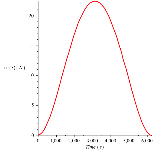
Fig. 3. Continuous control strategy for the input vector field V_1 = \mathbb{T}_1 to realize the straight-line transect.
