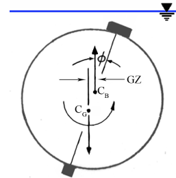
Fig. 1. Potential forces acting at C_G and C_B and the righting arm for a submerged spherical vehicle.
