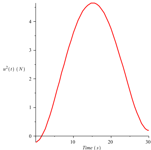
Fig. 5. Continuous control strategy for u^2 for the input vector field V_2 = 10T_5 to realize the turn-around.
