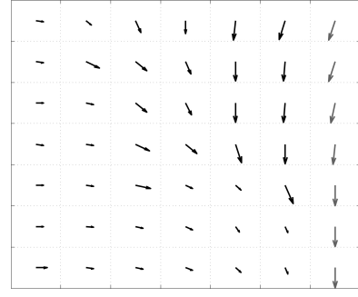
Fig. 6. Wind field distribution for Case 1. Arrow heads show the direction of the wind, and arrow lengths represent the magnitude of the wind (5 – 15 m/s).
