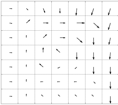
Fig. 8. Wind field distribution for case 2, where the head of arrows show the direction of the wind and the length of the arrows show the magnitude (5 – 15 m/s).
