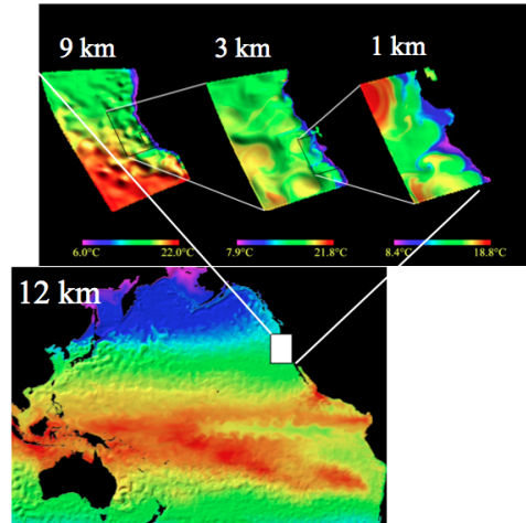
Fig. 1. An example output of a sea-surface temperature prediction for each of the available nested grids (resolutions of 12, 9, 3 and 1 km) from the ROMS run by the Jet Propulsion Laboratory. Image courtesy of Yi Chao, Jet Propulsion Laboratory.
