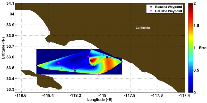
Fig. 7. A heat-map surface plot representing the normalised error between the surfacing location and the prescribed waypoint for the simulated trials.
