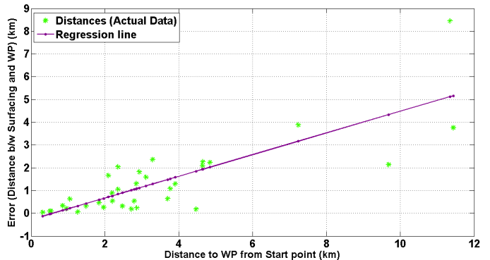
Fig. 3. A plot of the absolute surfacing error (in km) versus the length of the prescribed trajectory for the actual field trials.
