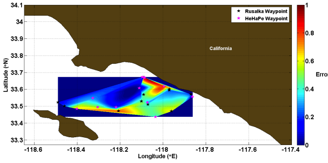
Fig. 4. A heat-map surface plot representing the normalised error between the surfacing location and the prescribed waypoint for the actual field trials.
