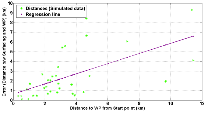
Fig. 6. A plot of the absolute surfacing error (in km) versus the length of the prescribed trajectory for the simulated trials.
