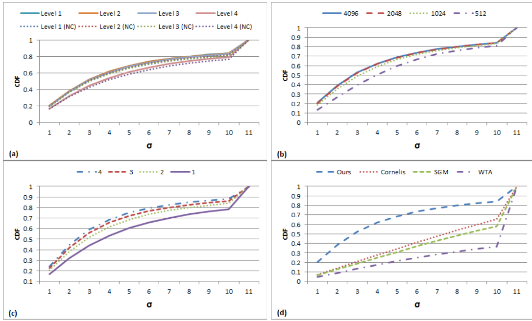
Fig. 4. Cumulative Distribution Function of estimates where the error is < n\sigma . (a) Adjusting the number of hierarchical levels ( k_l ) with and without (NC) depth-consistency (dashed). (b) Sweeping d_{inc} . (c) Adjusting the number of comparison views M . (d) Comparison with WTA, SGM and Cornellis.
