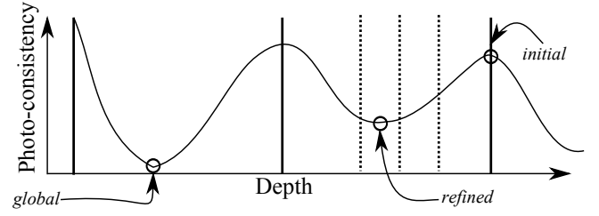
Fig. 2. Example of the photo-consistency cost function for a pixel. The locations of the discrete depth evaluations are indicated (bold vertical lines), as well as the global minimum, refined (parabolic) update and the initial (discrete) depth evaluation.
