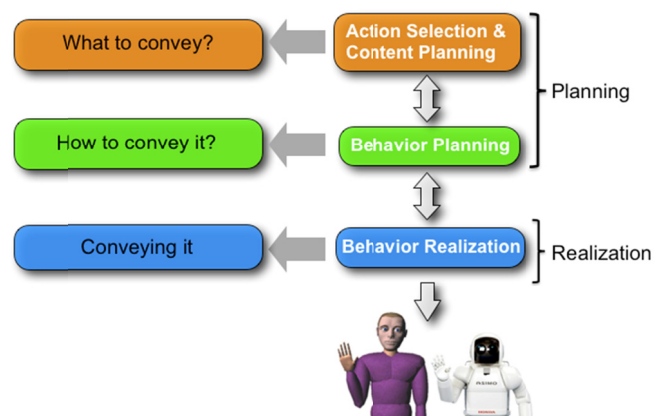
Figure 1. Behavior generation pipeline comprising two main stages: planning and realization (adapted from [9]).
