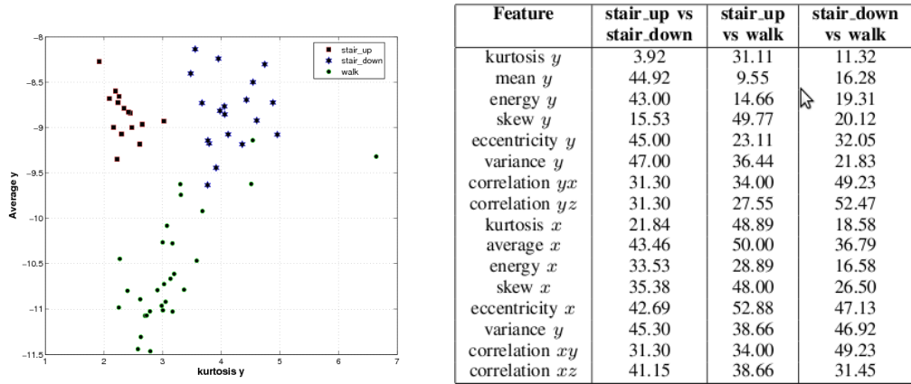
Fig. 5: Cluster plot and Misclassification rate of features
