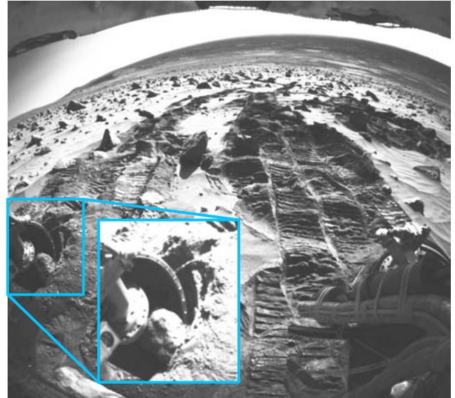
Figure 7: Rear HazCam image showing "Potato" rock stuck in the right rear wheel (inset). Note disturbed soil due to high slip while driving diagonally up the sandy slope.
