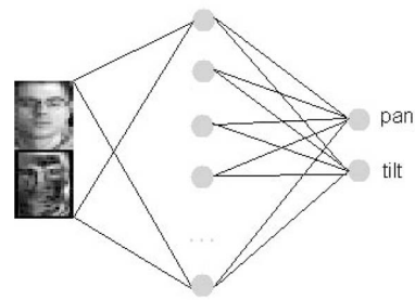
Fig. 4. Neural network for head-pose estimation. As input features, an intensity image of the head region and its Sobel magnitude are used.
