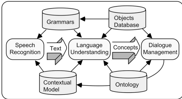
Fig. 5. Dialogue processing framework.
