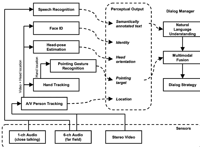
Fig. 2. Overview of the perceptual components.
