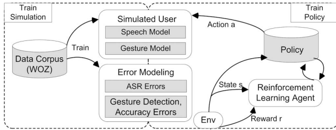
Fig. 10. RL with user simulation and error models.
