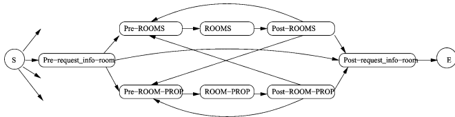
Fig. 6. Example of a schema for the speech act request_information-room. Nodes in rounded boxes are modeled with n -gram LMs, nodes in angled boxes with CFGs.
