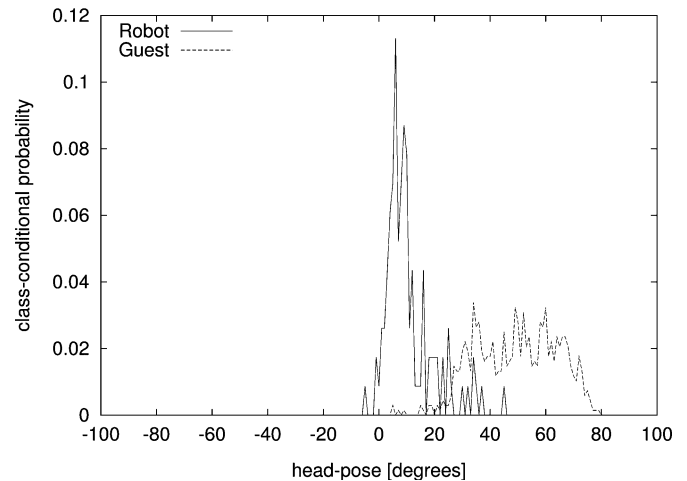
Fig. 8. Typical class-conditional probability distribution for the classification of the visual target for two targets.
