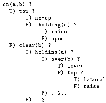
Figure 6: Decision tree form of stack(a,b) .
