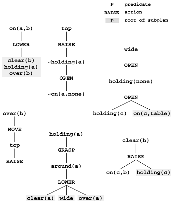
Figure 4: Part of the universal plan for stack(a,b) .
