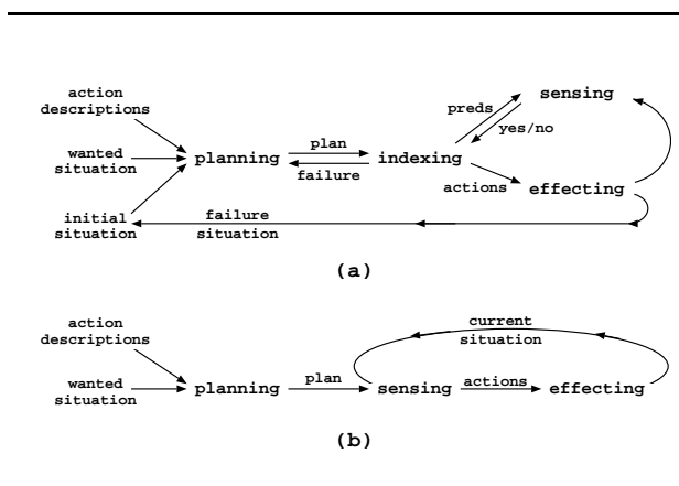
Figure 1: Plan monitoring vs planned reaction.
