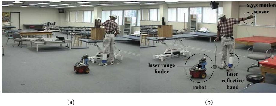
Figure 2: Two hands-off robot-assisted rehabilitation tasks: (a) magazine stacking and (b) free movement of the stroke-affected limb.
