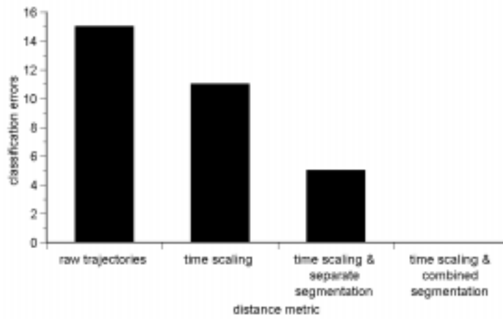
Fig. 3. Incorrect classifications (out of 60) made by the four variants of the metric
