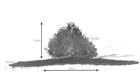
(b) Profile view of a semi-dwarf apple tree at the edge of a row of trees. The 3-D point cloud was reconstructed through the sensor suite, and illustrates the tree dimensions.
