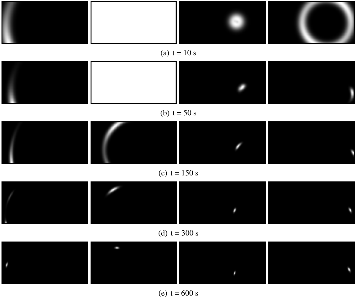
Figure 6: Example likelihood map progression using GPLVM path for the nodes in Fig. 4 ( 60 m \times 30 m loop). The left-to-right columns in this figure correspond to the left-to-right sequence of nodes (brown, blue, green, magenta) on the map. The estimates quickly become range annuli centered around the middle of the map (the moving node's starting location) and later collapse into a single mode as more range measurements are incorporated. Measurements are not received from the middle-left node until t = 150 s. Thus, the estimate is a uniform distribution until that time.
