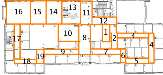
Figure 1: Discretization of office environment used for ranging radio tracking. The discretization uses structural aspects of the built environment to provide a room-level tracking with very noisy measurements.
