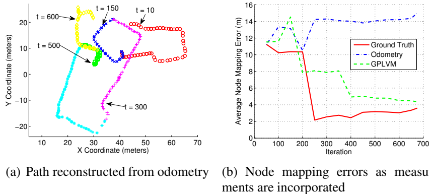
Figure 5: Comparison of path and node reconstruction for the GPLVM method and a method using only odometry in the 60\text{ m} \times 30\text{ m} environment. Drift in the path from odometry prevents the nodes from being accurately mapped. The GPLVM method does not use any odometry to reconstruct the path or the node locations.
