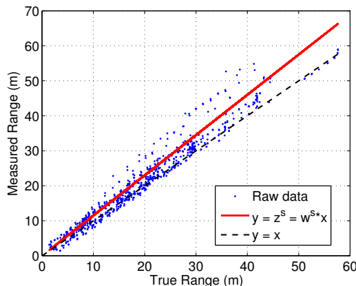
Figure 3: Noise model from using the mixture of Gaussians model where z^s = \hat{z}^* and w^s = \sum_i^{|\Gamma|} \omega_i s_i .
