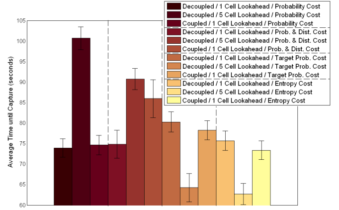
Fig. 5. Average simulated pursuit-evasion capture times for two pursuers over 1000 trials for coupled and decoupled coordination strategies with different cost heuristics on a complex office map. All methods used dispersion matrices. Lookahead trials with coupled planning were not feasible on this map. Error bars represent one standard error of the mean (SEM). See footnote for results of random and stationary strategies. Starting location of the evader was randomized, and starting locations of the pursuers were fixed.
