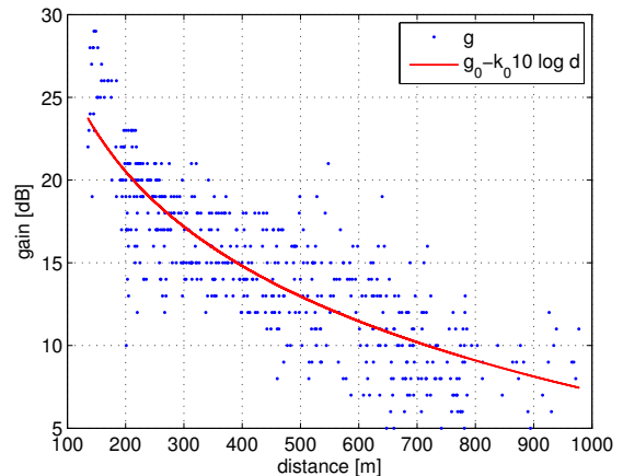
Fig. 1. Gain (normalized) vs. transmission distance. Dots show measured values; solid curve shows an estimated trend (a first-order logarithmic-scale polynomial fit to the ensemble mean at each distance yields k_0=1.9 ).
