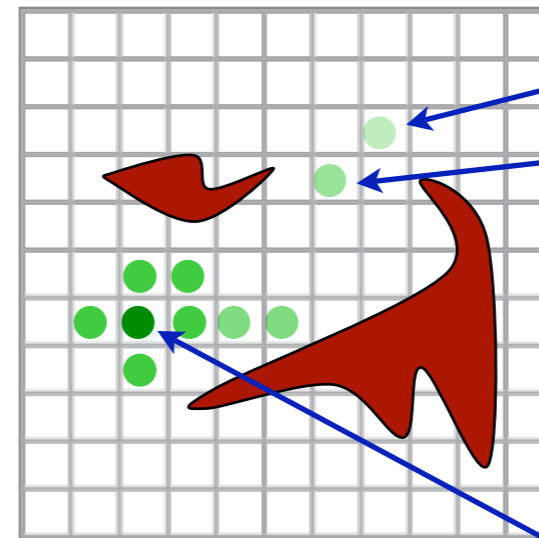
POMDP planning
