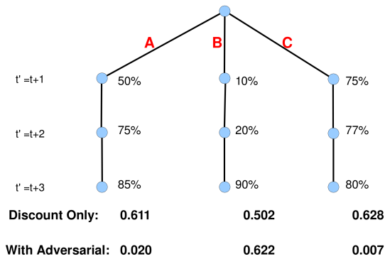
Fig. 4. Sample trajectories and the associated rewards. A pursuer is choosing among three candidate sequences of action. Each node is labeled with an estimate of P_{cr} , the probability that, for that depth, the evader will be captured given the random motion assumption. The cumulative reward for each trajectory is shown both with and without the assumption that the evaders are adversarial. S = 20 , \gamma = .8
