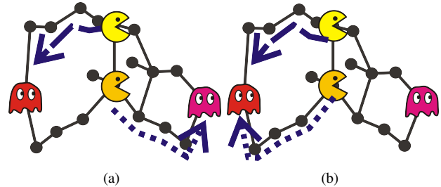
Fig. 1. (a) Previous probabilistic pursuit methods assumed random evaders. (b) We show how to extend this model to adversarial evaders which require more teamwork to catch.
