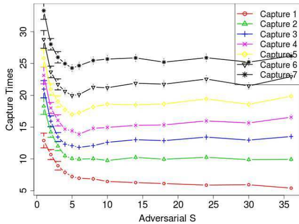
Fig. 9. Pursuit of a marginally adversarial evader (minimax depth one) on the CDG graph. Experiments like this one can be used to determine S experimentally. In this case, the minimum at S \approx 4 indicates the optimal S for minimax adversaries of depth one.
