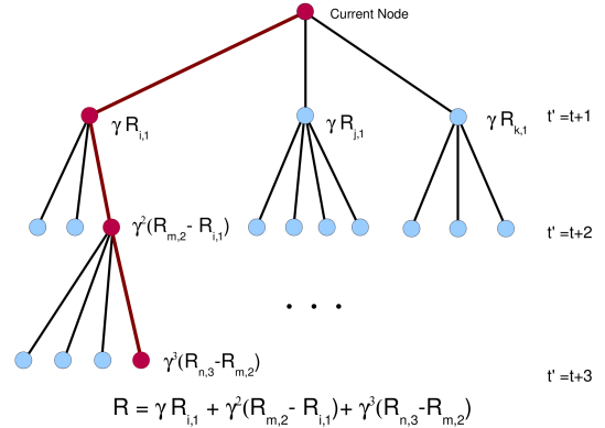
Fig. 2. Discounted rewards as depth increases. The immediate reward is discounted by \gamma^d and the total reward for a plan is the sum of incremental rewards along the path. The value of R_{i,t} corresponds to the cumulative reward at node i at time t . If at any node the total possible reward for continuing down this path is less than \epsilon the rest of that path will be pruned.
