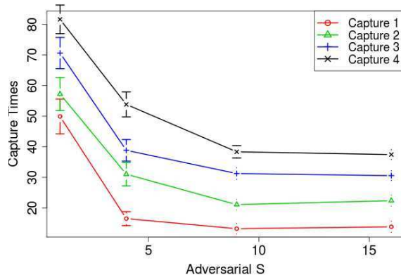
Fig. 8. For comparison, we validate our model by running 2 pursuers on the museum graph against 5 evaders running a fixed depth mini-max search with alpha-beta pruning. For this trial, the evader depth was limited to 4 for computational reasons. This graph shows matching trends to Figure 7, and provides a baseline for comparison to our 100-sample agent.
