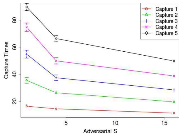
Fig. 7. On the museum graph 5b, capture time decreases significantly as the pursuers’ model of the evader more accurately reflects their adversarialness. S = 1 corresponds to the random evader considered in Hollinger’s work, while higher S correspond to explicitly modeling the evaders as adversarial. In this trial, two pursuers team up to capture five independently adversarial evaders. Error bars reflect one standard error of the mean.
