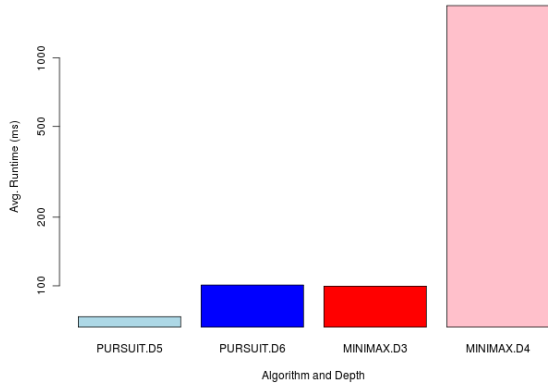
Fig. 6. Comparative run times (log-scale) of the pursuers’ algorithm (blue) and the evaders’ minimax algorithm (red) to varying depths. Note that our algorithm searches to a depth of 6 timesteps in the same time that minimax searches to a depth of 3.
