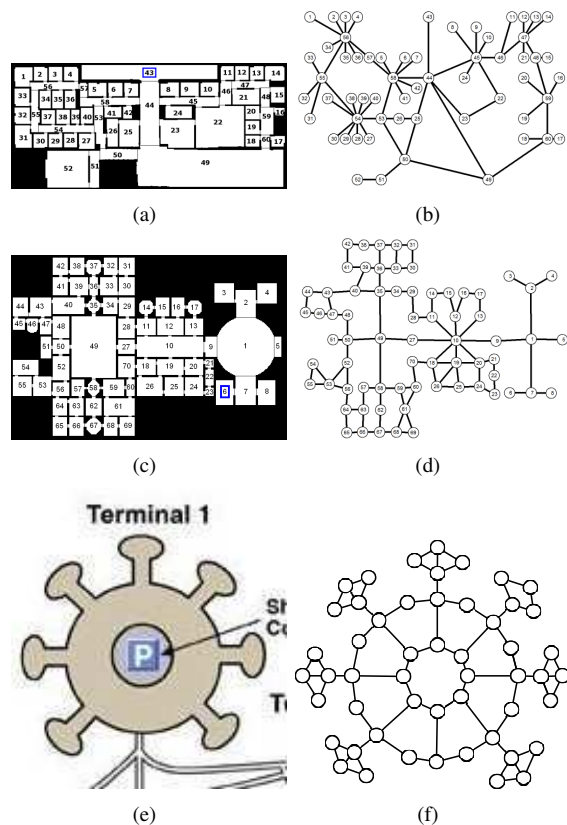
Fig. 5. Map and graph pairs used in this project. The graphs of Newell-Simon Hall at Carnegie Mellon University (a) and the US National Gallery Museum (c), were introduced by Hollinger and offer a good benchmark since these have been used in previous work. We also introduce a more uniformly complex map of the Charles de Gaulle airport in Paris (e).
