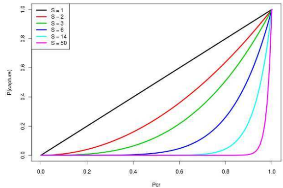
Fig. 3. The effect of the adversarial skill parameter S on expected probability of capture, given the probability of capture P_{cr} from the random diffusion model in [4]. (See Equation 2.)
