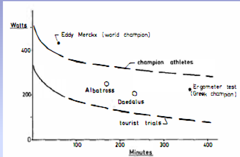
Figure 2 Human-power output vs. duration of effort.
