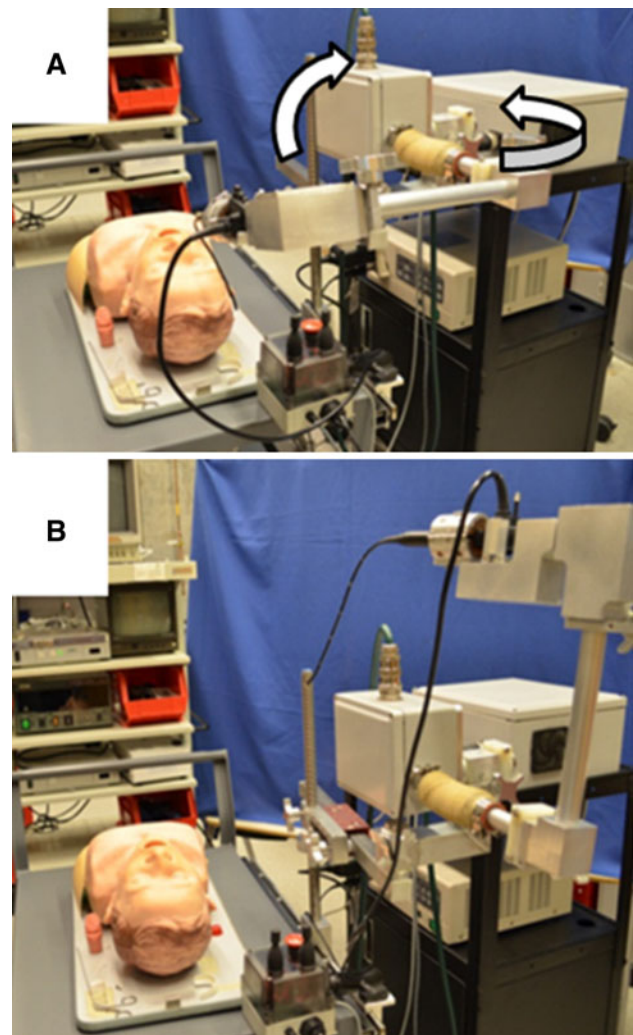
Fig. 3 The scope can be quickly removed from the vicinity of the patient by using the passive elbow joint on the robot arm. a Rotate the knob and raise the arm. b The arm has been raised
