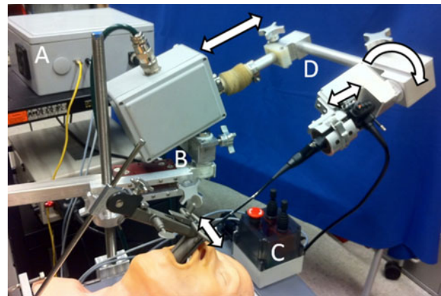
Fig. 1 Robotic EndoLaryngeal (Robo-ELF) Scope System. A Electronics enclosure, B five degree of freedom positioning arm, C joystick enclosure, D robot system
