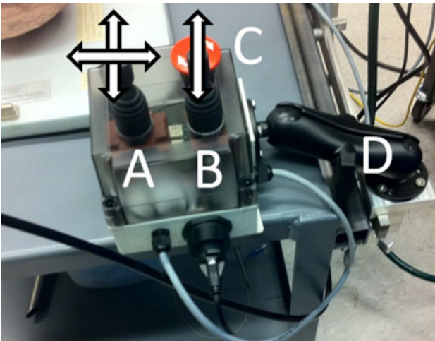
Fig. 4 Joystick enclosure. A Two degree of freedom joystick, B one degree of freedom joystick, C emergency off button, D joystick positioning arm
