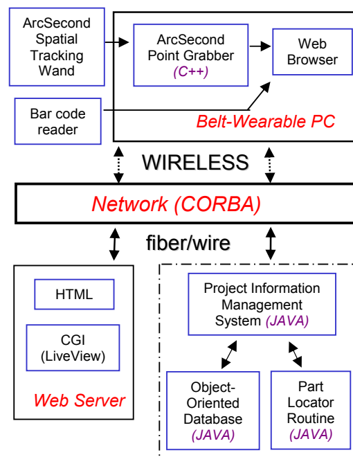
Figure 1. System architecture developed for the prototype implementation.
