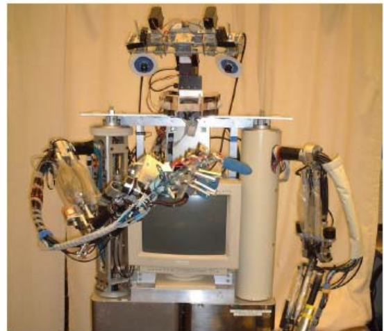
Figure 1. ISAC, a humanoid upper torso, equipped with two six-DOF McKibben actuated arms, anthropomorphic end-effectors called PneuHands, a four-DOF stereovision head, voice recognition, and a monitor for graphical display.
