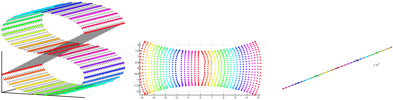
Figure 2: “S”-curve trajectory example motivated by Roweis and Saul. (top) Plot of 3D trajectory of a point moving along an S-Curve with its temporal order specified by the dashed line. The point traverses the S and returns to its initial position along the “S”, shifted slightly off of the previous S. (middle) The embedding produced by spatial Isomap removes the spatial nonlinearity of the S. (bottom) The embedding produced by spatio-temporal Isomap removes the spatial nonlinearity and collapses the multiple traversals of the S to a line.
