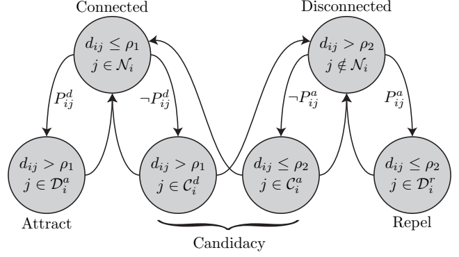
Fig. 2. Model for discriminative connectivity, including signals and switching states for link addition and deletion, where d_{ij} \triangleq \|x_{ij}\| .
