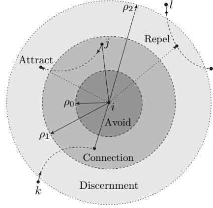
Fig. 1. Agent interaction model with radii determining sensing and communication \|x_{ij}\| \leq \rho_2 , neighbor discernment relative to constraints \rho_1 < \|x_{ij}\| \leq \rho_2 , link establishment \|x_{ik}\| \leq \rho_1 , and collision avoidance \|x_{ij}\| \leq \rho_0 .
