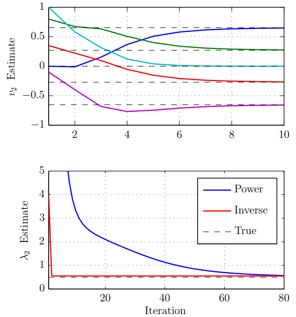
Fig. 3. Distributed inverse iteration for algebraic connectivity estimation: (top) per-agent convergence of the components of v_2 associated with 5-agent test network (not shown); (bottom) \lambda_2 estimate convergence for inverse iteration vs. power iteration over 50-agent test network (not shown).
