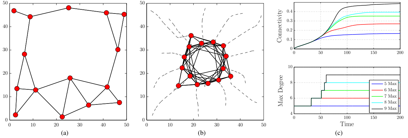
Fig. 4. Aggregation simulation of a 15-agent system with connectivity maximization under degree constraint |\mathcal{N}_i| \leq 9 , with interaction radii \rho_2 = 20 , \rho_1 = 18 , and \rho_0 = 5 : (a) random initial configuration; (b) final converged configuration with agent paths (dashed); (c) algebraic connectivity (top) and maximum degree (bottom) over varying degree constraints (illustrated |\mathcal{N}_i| \leq 9 bound shown in black).
