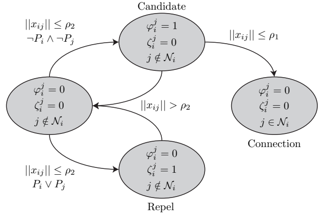
Fig. 2. Model for discriminative connectivity, including signals and associated switching conditions for controlling link addition.
