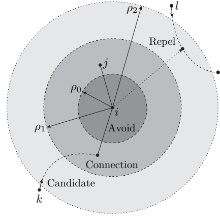
Fig. 1. Agent interaction model. Agents can sense one another and willfully communicate within the interaction radius \rho_2 . In the discernment region, \rho_1 < \|x_{ik}\| \leq \rho_2 , agents determine, relative to local constraints, whether nearby agents are candidates for connection (agent k ) or should be repelled (agent l ) due to constraint violation. In the connection region with radius \rho_1 < \rho_2 , agents establish communication, where collision avoidance is activated within a radius \rho_0 < \rho_1 .
