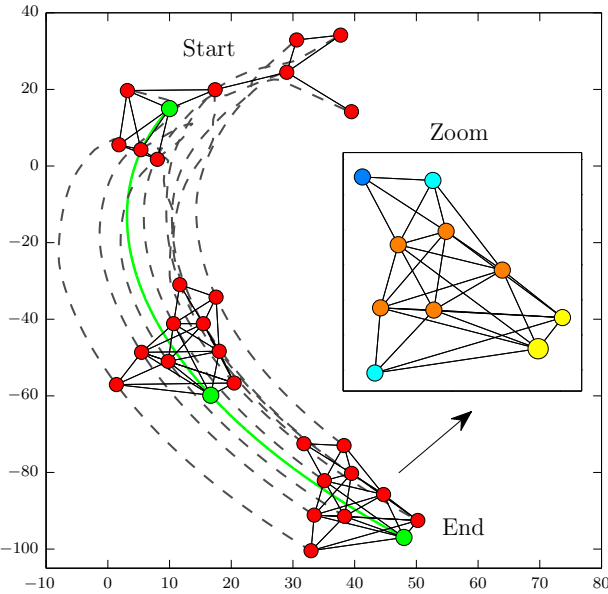
Fig. 5. Leader-following simulation, with n = 10 , connectivity maximization under |\mathcal{N}_i| \leq 7 , and interaction radii \rho_2 = 20 , \rho_1 = 18 , \rho_0 = 5 . The leader and its path (green), and agent configurations during execution are composited, along with a zoom of the final configuration with node degree highlighted.
