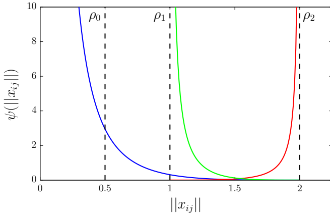
Fig. 4. Composite of inter-agent potentials for constrained dispersion, including dispersion (blue, j \in \mathcal{N}_i ), link retention (red, j \in \mathcal{D}_i^a ), and link denial (green, j \in \mathcal{D}_i^r ). The interaction model parameters \rho_2, \rho_1, \rho_0 are illustrated by dashed lines.
