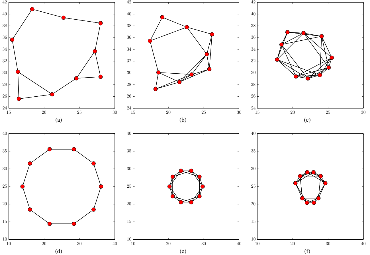
Fig. 5. Aggregation simulations of an n = 10 agent system with interaction model \rho_2 = 10 , \rho_1 = 7 , and \rho_0 = 2 , under maximum degree constraints |\mathcal{N}_i| \leq 6 [(a)-(c)] and |\mathcal{N}_i| \leq 5 [(d)-(f)]: (a) random initial configuration; (b) intermediate configuration |\mathcal{N}_i| \leq 6 ; (c) final converged configuration |\mathcal{N}_i| \leq 6 ; (d) initial ring network configuration; (e) final converged configuration |\mathcal{N}_i| \leq 4 ; and (f) final converged configuration |\mathcal{N}_i| \leq 5 .
