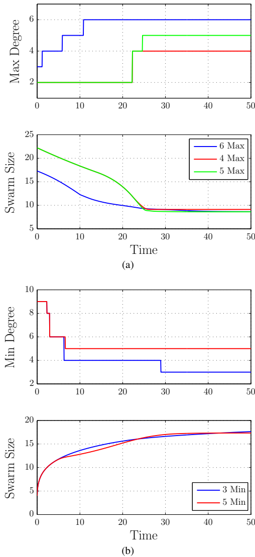
Fig. 7. Node degree bounds and swarm size for aggregation and dispersion simulations depicted in Figs. 5 and 6: (a) maximum node degree (top) and swarm size (bottom) for |\mathcal{N}_i| \leq 6 (blue, [Fig. 5c]), |\mathcal{N}_i| \leq 4 (red, [Fig. 5e]), and |\mathcal{N}_i| \leq 5 (green, [Fig. 5f]); and (b) minimum node degree (top) and swarm size (bottom) for |\mathcal{N}_i| \geq 3 (blue, [Fig. 6c]) and |\mathcal{N}_i| \geq 5 (red, [Fig. 6b]).
