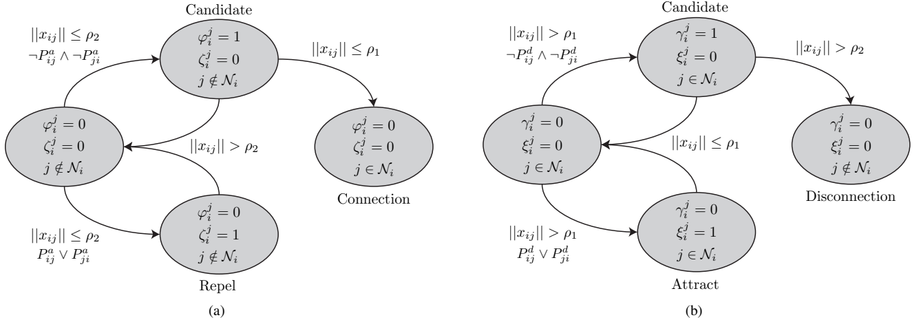
Fig. 2. Model for discriminative connectivity, including signals and associated switching conditions for controlling: (a) link addition; (b) link deletion.
