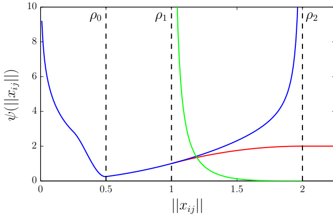
Fig. 3. Composite of inter-agent potentials for constrained aggregation, including aggregation, collision avoidance, and link retention (blue, j \in \mathcal{N}_i ), link denial (green, j \in \mathcal{D}_i^r ), and continuity-preserving attraction (red, j \in \mathcal{C}_i^a ). The interaction model parameters \rho_2, \rho_1, \rho_0 are illustrated by dashed lines.
