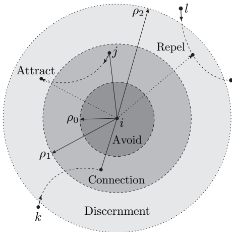
Fig. 1. Agent interaction model. Agents can sense one another and communicate within the interaction radius \rho_2 . In the discernment region, \rho_1 < \|x_{ij}\| \leq \rho_2 , an agent ( i ) determines, relative to local constraints, whether adjacent agents are candidates for link addition ( k ) or removal, or should be attracted ( j ) or repelled ( l ) due to constraint violation. In the connection region with radius \rho_1 < \rho_2 , agents establish communication, with collision avoidance being activated within a radius \rho_0 < \rho_1 .
