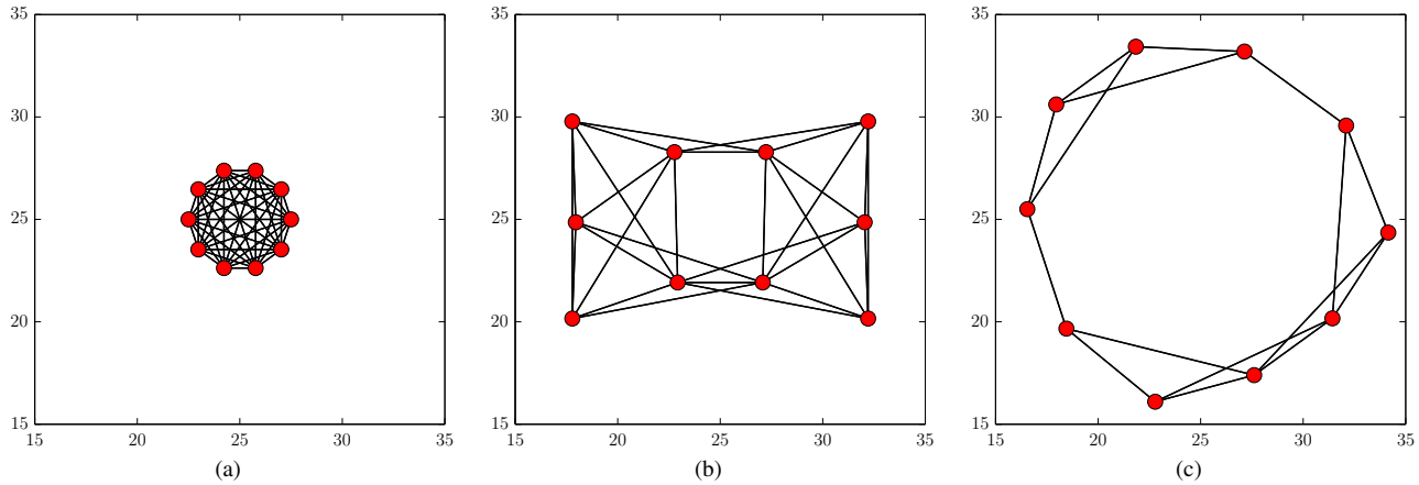
Fig. 6. Dispersion simulations of an n = 10 agent system with interaction model \rho_2 = 10 , \rho_1 = 7 , and \rho_0 = 2 , under minimum degree constraints |\mathcal{N}_i| \geq 5 [(b)] and |\mathcal{N}_i| \geq 3 [(c)]: (a) initial fully connected ring network configuration; (b) final converged configuration |\mathcal{N}_i| \geq 5 ; and (c) final converged configuration |\mathcal{N}_i| \geq 3 .
