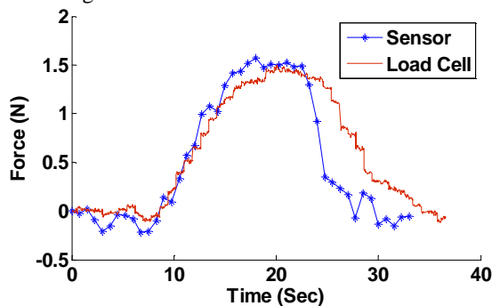
Figure 6: Above) Normal force sensor vs. force-plate output after calibration trials
